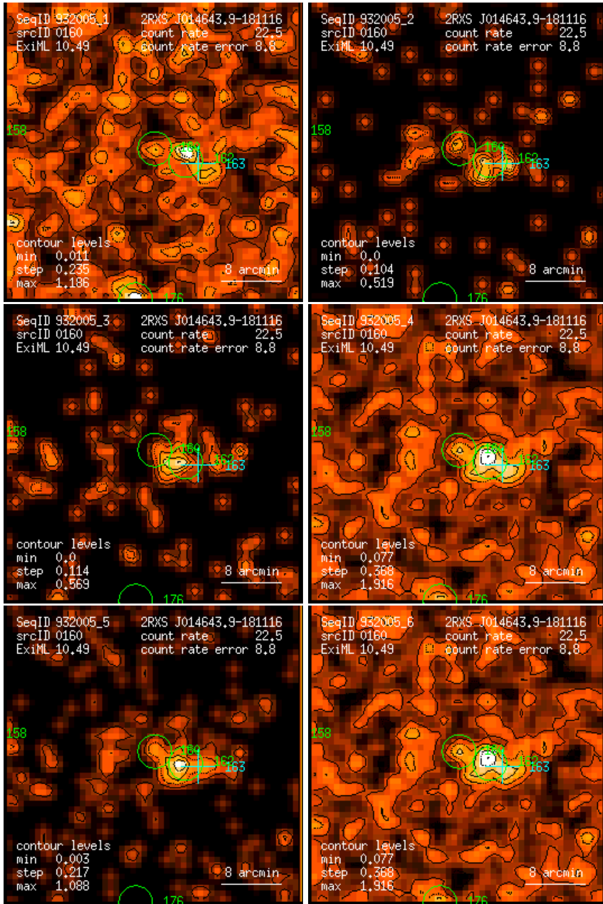
Figure 160: RASS 932005: detection 0160: band rate images, Gaussian filter: (1) PSPC channels 11 – 41, (2) 52 – 90, (3) 91 – 201, (4) 11 – 235, (5) 52 – 201, (6) 11 – 201. Broad band rates in counts/ks. Band rate contour levels in counts/ks/arcmin 2 .
