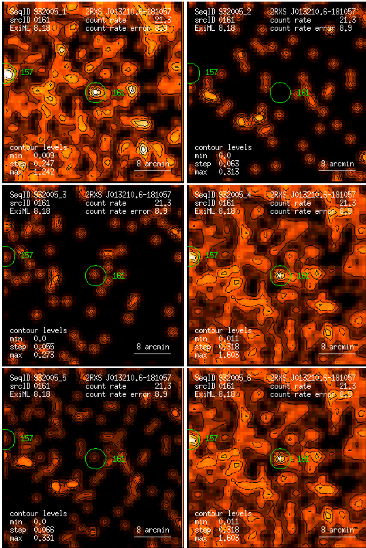
Figure 161: RASS 932005: detection 0161: band rate images, Gaussian filter: (1) PSPC channels 11 – 41, (2) 52 – 90, (3) 91 – 201, (4) 11 – 235, (5) 52 – 201, (6) 11 – 201. Broad band rates in counts/ks. Band rate contour levels in counts/ks/arcmin 2 .
