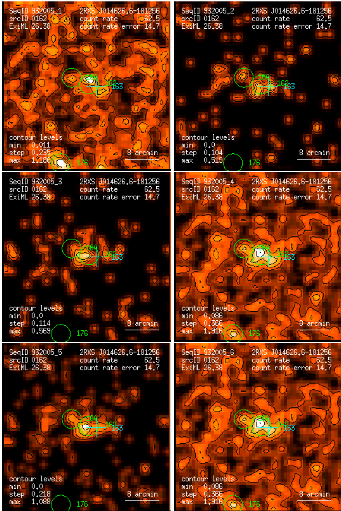
Figure 162: RASS 932005: detection 0162: band rate images, Gaussian filter: (1) PSPC channels 11 – 41, (2) 52 – 90, (3) 91 – 201, (4) 11 – 235, (5) 52 – 201, (6) 11 – 201. Broad band rates in counts/ks. Band rate contour levels in counts/ks/arcmin 2 .
