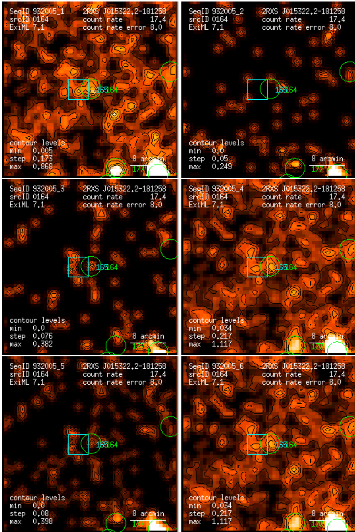
Figure 164: RASS 932005: detection 0164: band rate images, Gaussian filter: (1) PSPC channels 11 – 41, (2) 52 – 90, (3) 91 – 201, (4) 11 – 235, (5) 52 – 201, (6) 11 – 201. Broad band rates in counts/ks. Band rate contour levels in counts/ks/arcmin 2 .
