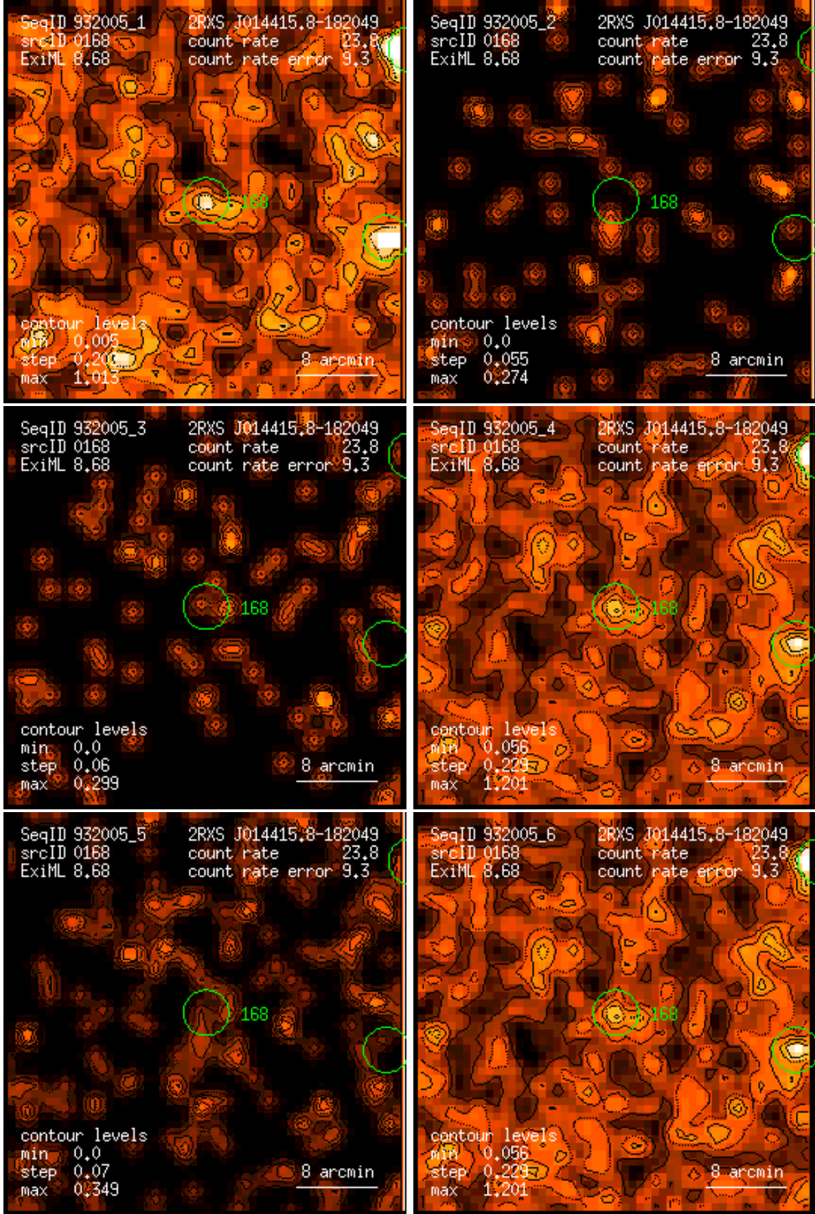
Figure 168: RASS 932005: detection 0168: band rate images, Gaussian filter: (1) PSPC channels 11 – 41, (2) 52 – 90, (3) 91 – 201, (4) 11 – 235, (5) 52 – 201, (6) 11 – 201. Broad band rates in counts/ks. Band rate contour levels in counts/ks/arcmin 2 .
