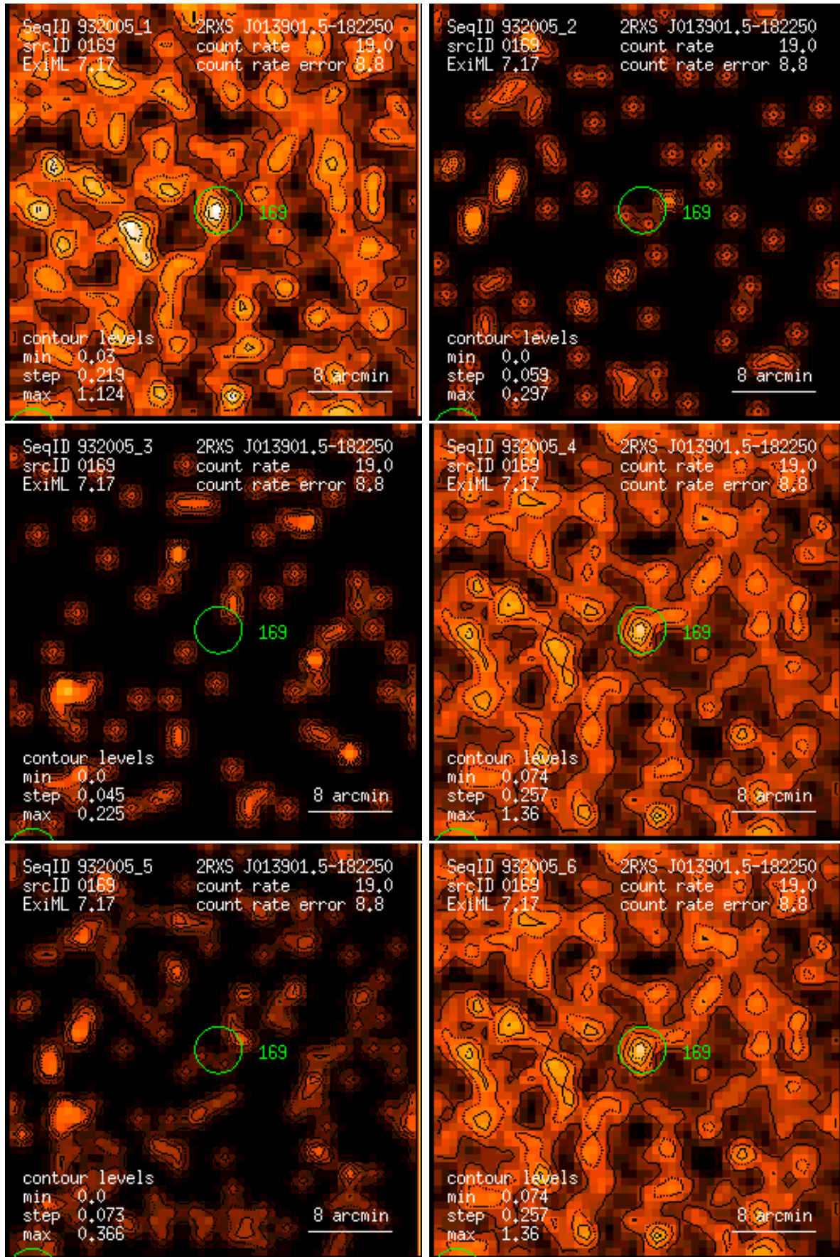
Figure 169: RASS 932005: detection 0169: band rate images, Gaussian filter: (1) PSPC channels 11 – 41, (2) 52 – 90, (3) 91 – 201, (4) 11 – 235, (5) 52 – 201, (6) 11 – 201. Broad band rates in counts/ks. Band rate contour levels in counts/ks/arcmin 2 .
