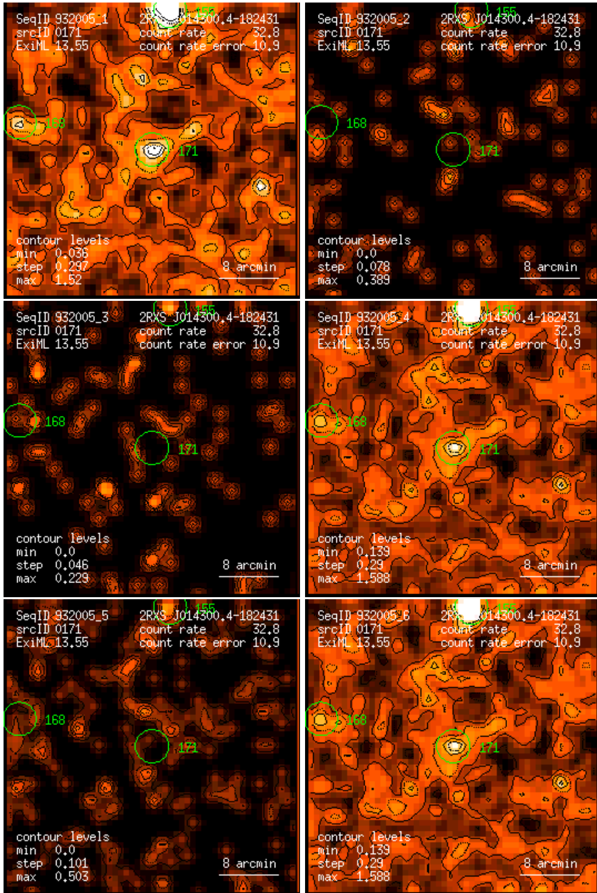
Figure 171: RASS 932005: detection 0171: band rate images, Gaussian filter: (1) PSPC channels 11 – 41, (2) 52 – 90, (3) 91 – 201, (4) 11 – 235, (5) 52 – 201, (6) 11 – 201. Broad band rates in counts/ks. Band rate contour levels in counts/ks/arcmin 2 .
