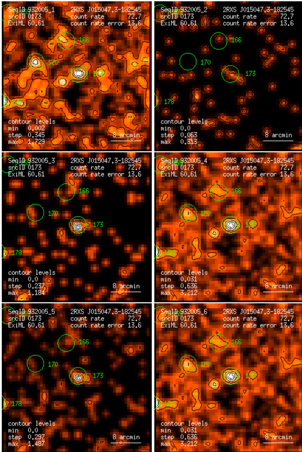
Figure 173: RASS 932005: detection 0173: band rate images, Gaussian filter: (1) PSPC channels 11 – 41, (2) 52 – 90, (3) 91 – 201, (4) 11 – 235, (5) 52 – 201, (6) 11 – 201. Broad band rates in counts/ks. Band rate contour levels in counts/ks/arcmin 2 .
