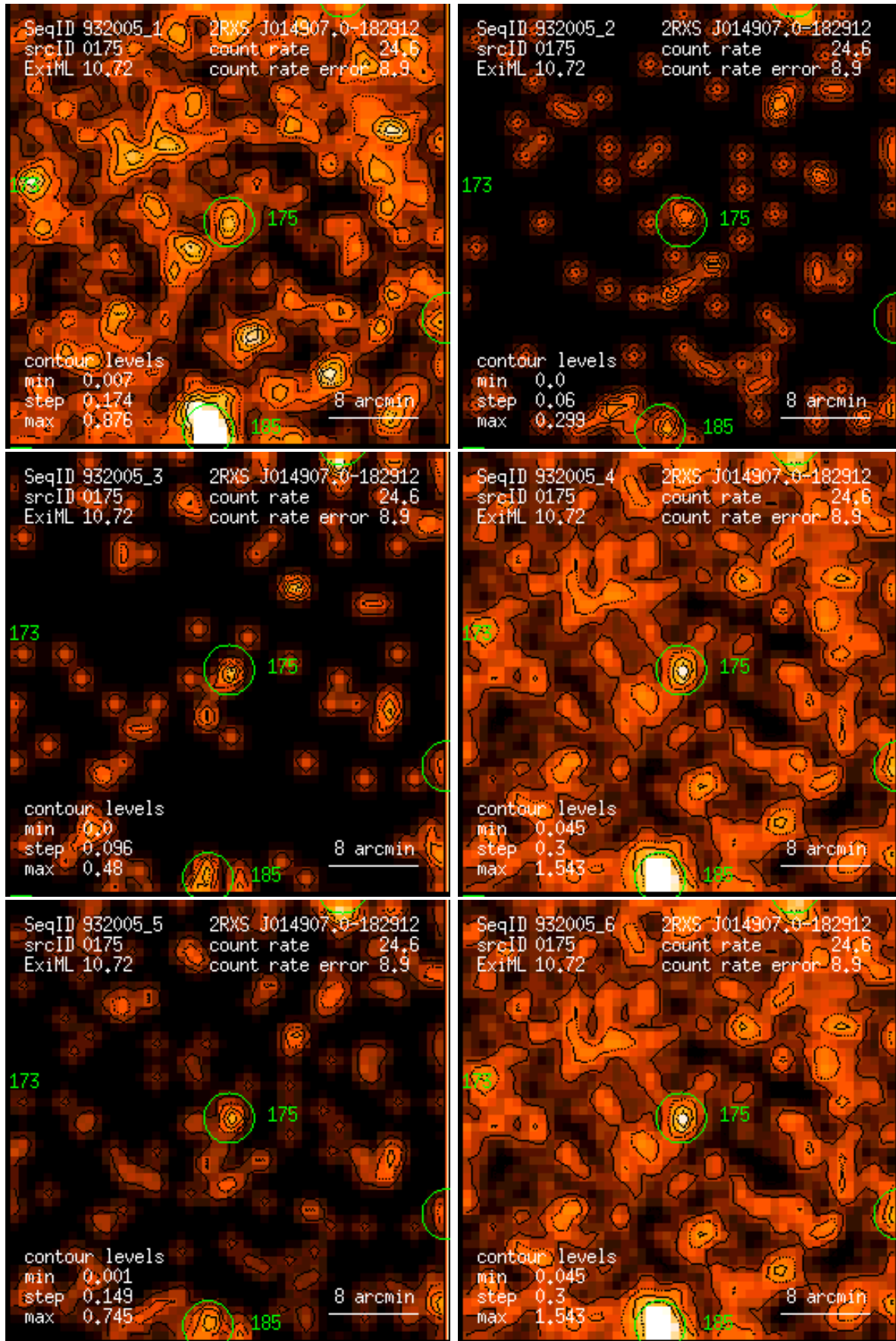
Figure 175: RASS 932005: detection 0175: band rate images, Gaussian filter: (1) PSPC channels 11 – 41, (2) 52 – 90, (3) 91 – 201, (4) 11 – 235, (5) 52 – 201, (6) 11 – 201. Broad band rates in counts/ks. Band rate contour levels in counts/ks/arcmin 2 .
