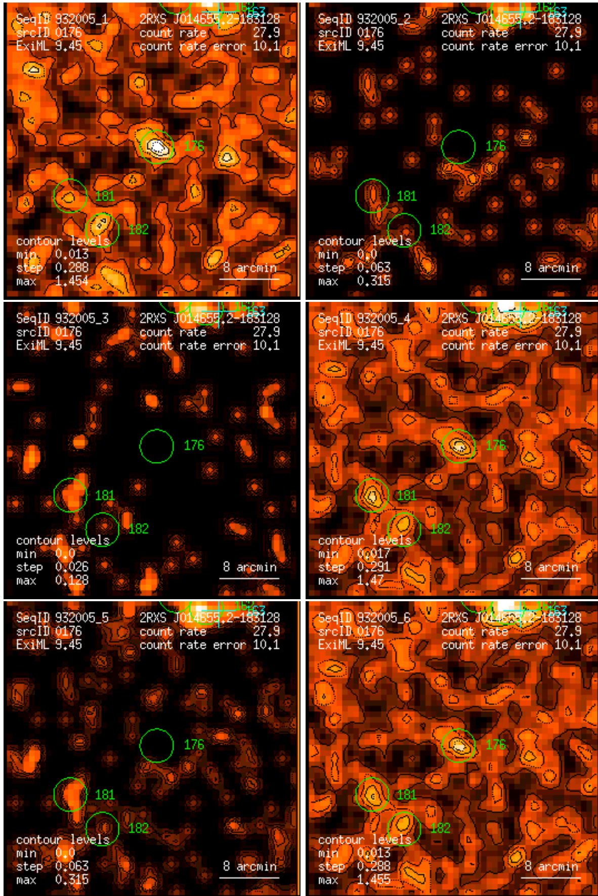
Figure 176: RASS 932005: detection 0176: band rate images, Gaussian filter: (1) PSPC channels 11 – 41, (2) 52 – 90, (3) 91 – 201, (4) 11 – 235, (5) 52 – 201, (6) 11 – 201. Broad band rates in counts/ks. Band rate contour levels in counts/ks/arcmin 2 .
