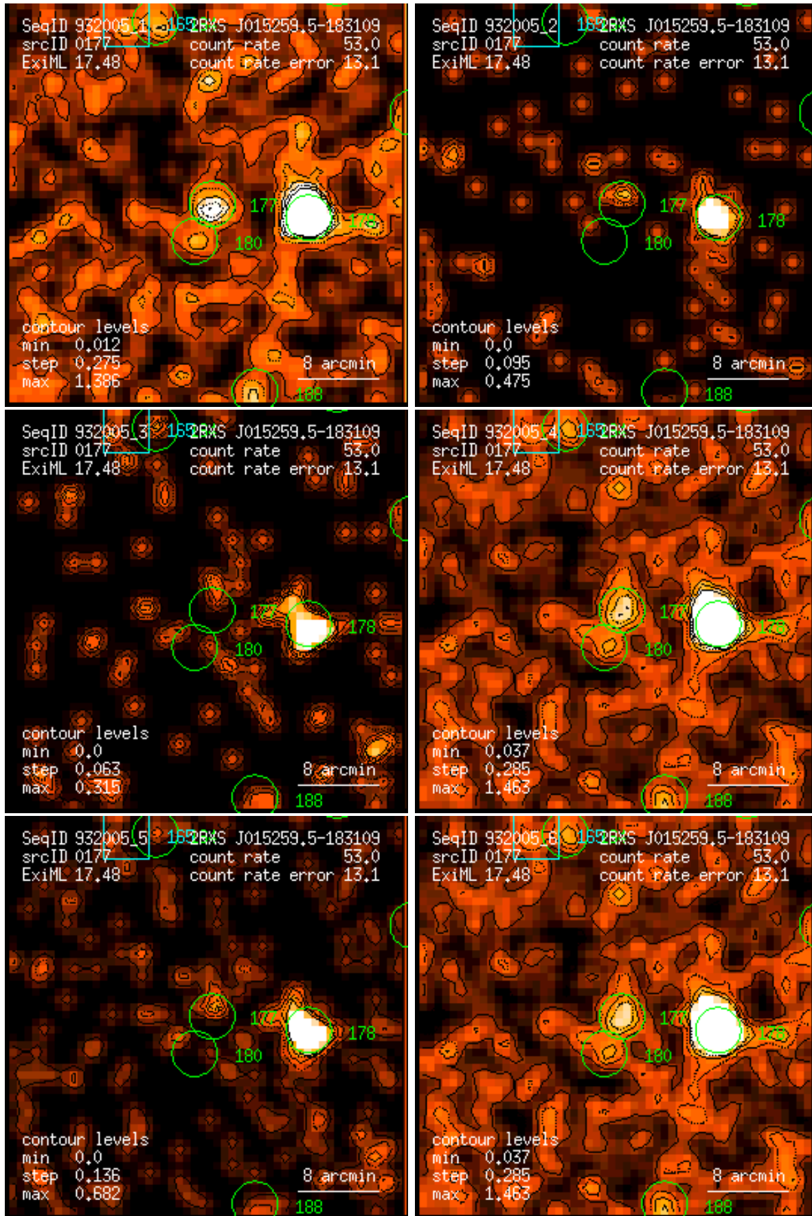
Figure 177: RASS 932005: detection 0177: band rate images, Gaussian filter: (1) PSPC channels 11 – 41, (2) 52 – 90, (3) 91 – 201, (4) 11 – 235, (5) 52 – 201, (6) 11 – 201. Broad band rates in counts/ks. Band rate contour levels in counts/ks/arcmin 2 .
