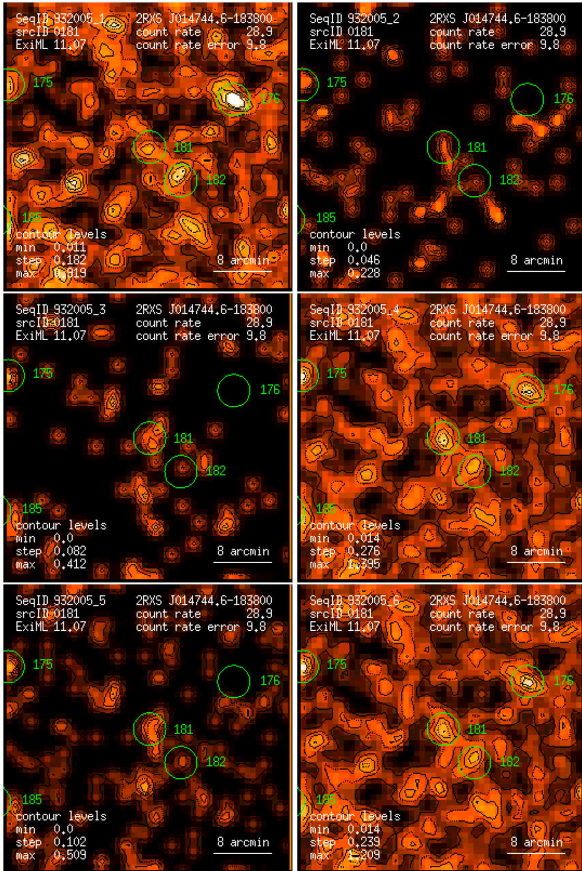
Figure 181: RASS 932005: detection 0181: band rate images, Gaussian filter: (1) PSPC channels 11 – 41, (2) 52 – 90, (3) 91 – 201, (4) 11 – 235, (5) 52 – 201, (6) 11 – 201. Broad band rates in counts/ks. Band rate contour levels in counts/ks/arcmin 2 .
