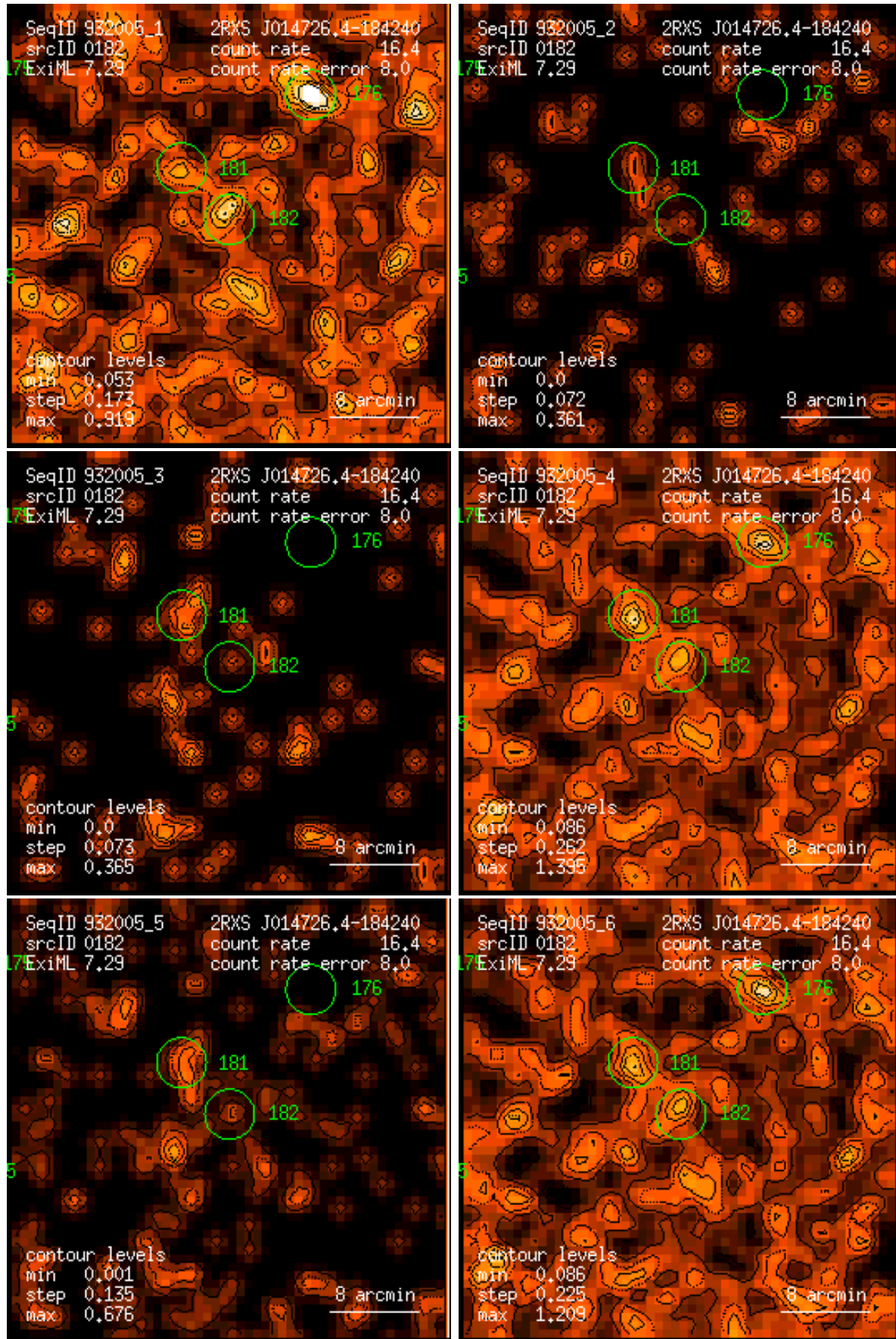
Figure 182: RASS 932005: detection 0182: band rate images, Gaussian filter: (1) PSPC channels 11 – 41, (2) 52 – 90, (3) 91 – 201, (4) 11 – 235, (5) 52 – 201, (6) 11 – 201. Broad band rates in counts/ks. Band rate contour levels in counts/ks/arcmin 2 .
