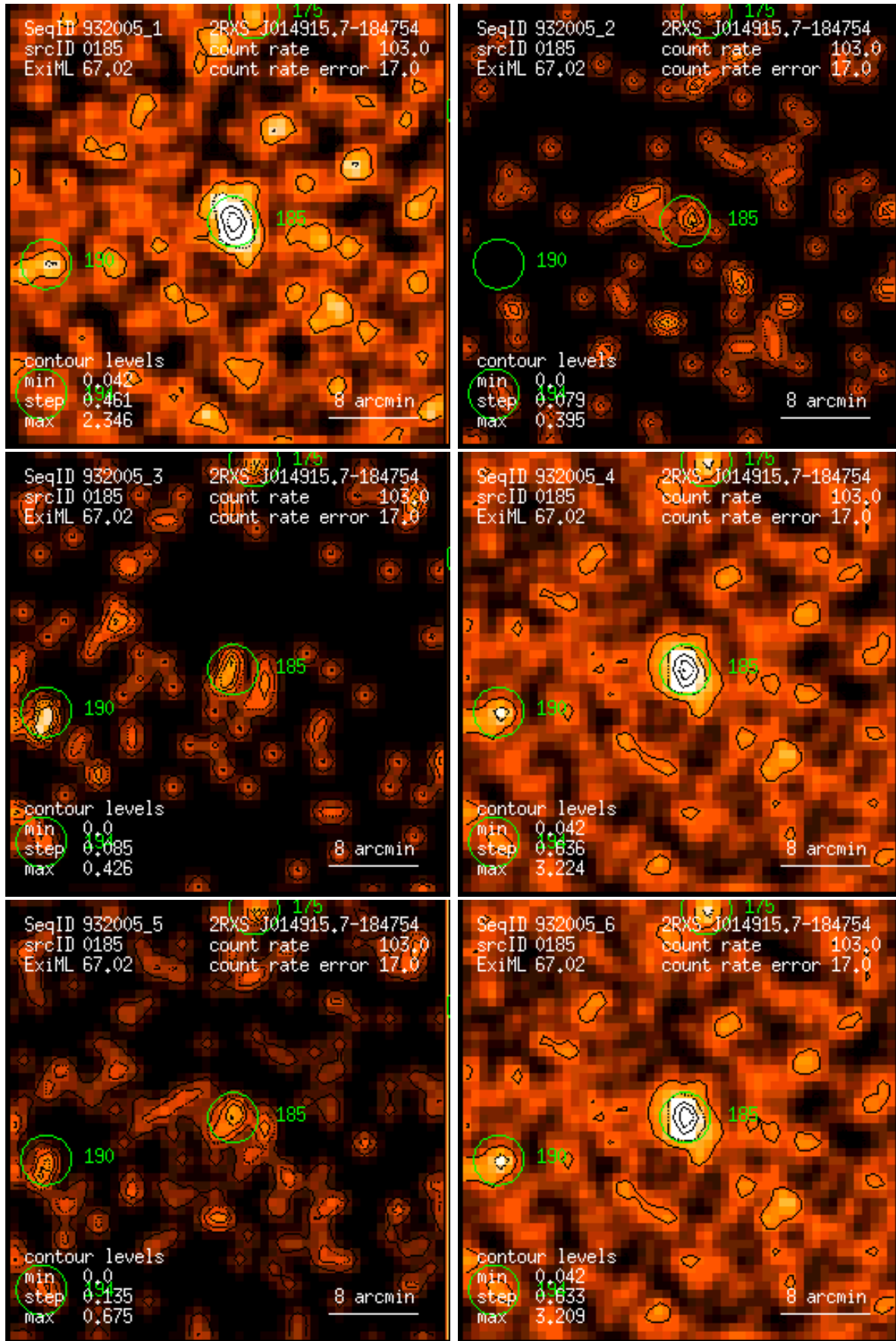
Figure 185: RASS 932005: detection 0185: band rate images, Gaussian filter: (1) PSPC channels 11 – 41, (2) 52 – 90, (3) 91 – 201, (4) 11 – 235, (5) 52 – 201, (6) 11 – 201. Broad band rates in counts/ks. Band rate contour levels in counts/ks/arcmin 2 .
