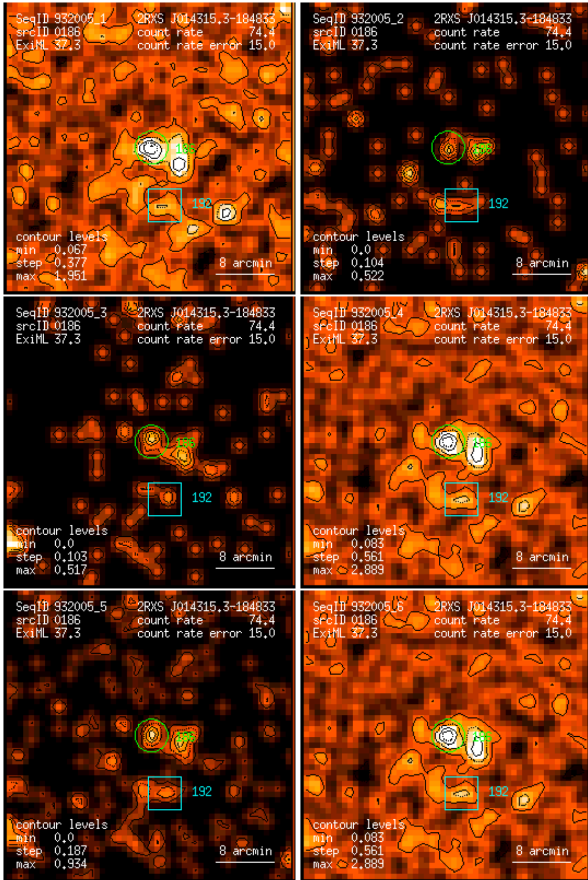
Figure 186: RASS 932005: detection 0186: band rate images, Gaussian filter: (1) PSPC channels 11 – 41, (2) 52 – 90, (3) 91 – 201, (4) 11 – 235, (5) 52 – 201, (6) 11 – 201. Broad band rates in counts/ks. Band rate contour levels in counts/ks/arcmin 2 .
