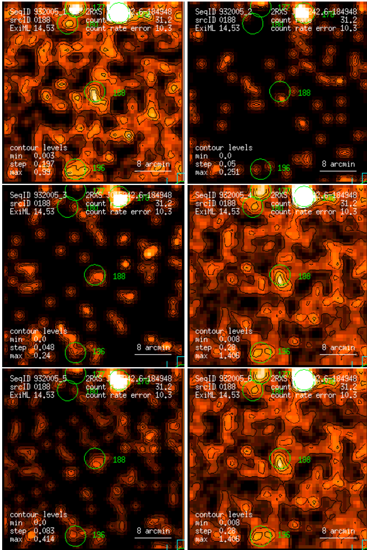
Figure 188: RASS 932005: detection 0188: band rate images, Gaussian filter: (1) PSPC channels 11 – 41, (2) 52 – 90, (3) 91 – 201, (4) 11 – 235, (5) 52 – 201, (6) 11 – 201. Broad band rates in counts/ks. Band rate contour levels in counts/ks/arcmin 2 .
