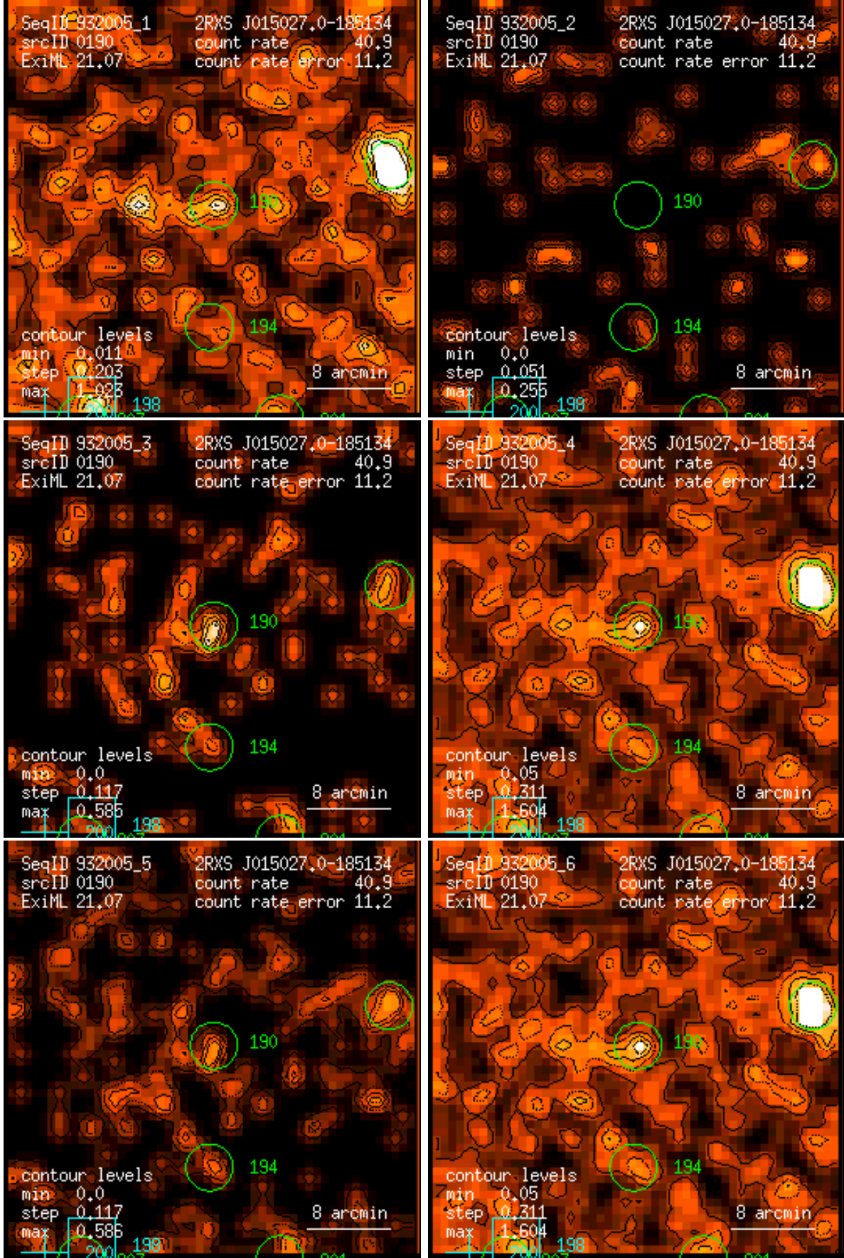
Figure 190: RASS 932005: detection 0190: band rate images, Gaussian filter: (1) PSPC channels 11 – 41, (2) 52 – 90, (3) 91 – 201, (4) 11 – 235, (5) 52 – 201, (6) 11 – 201. Broad band rates in counts/ks. Band rate contour levels in counts/ks/arcmin 2 .
