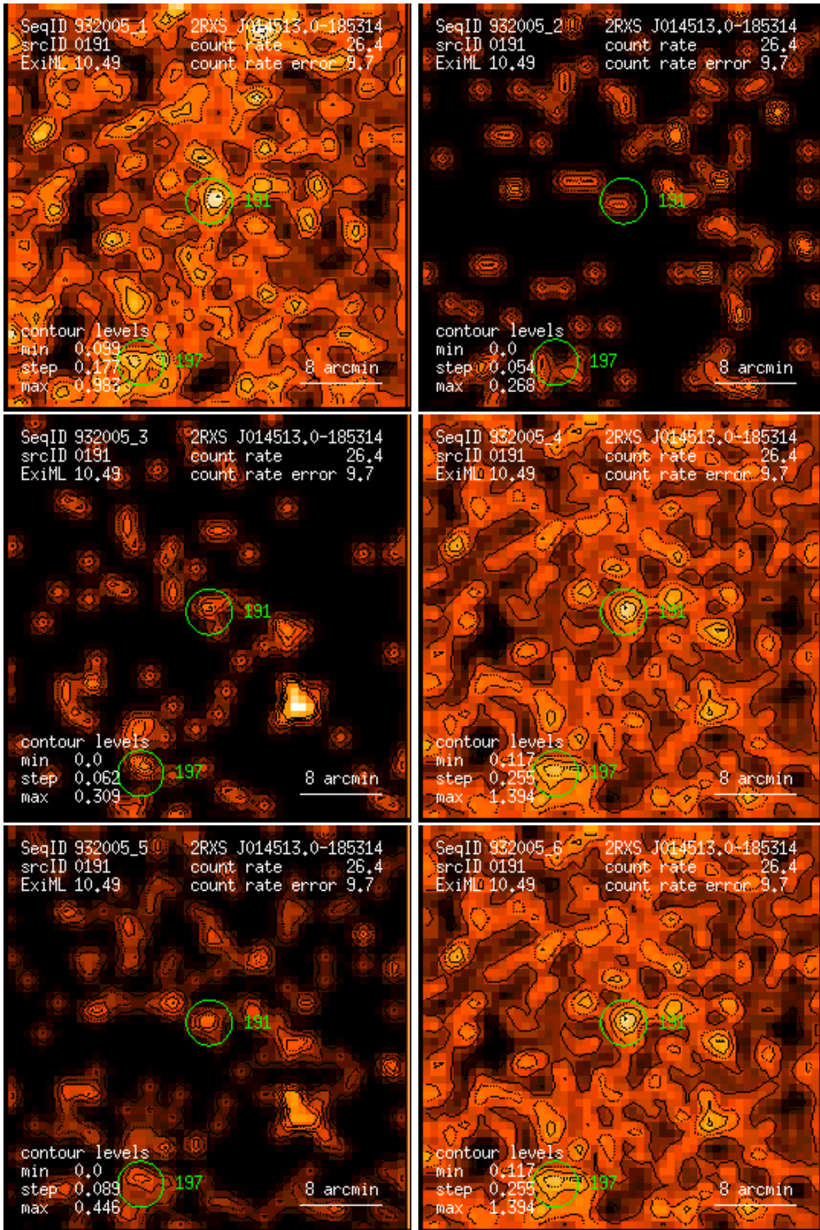
Figure 191: RASS 932005: detection 0191: band rate images, Gaussian filter: (1) PSPC channels 11 – 41, (2) 52 – 90, (3) 91 – 201, (4) 11 – 235, (5) 52 – 201, (6) 11 – 201. Broad band rates in counts/ks. Band rate contour levels in counts/ks/arcmin 2 .
