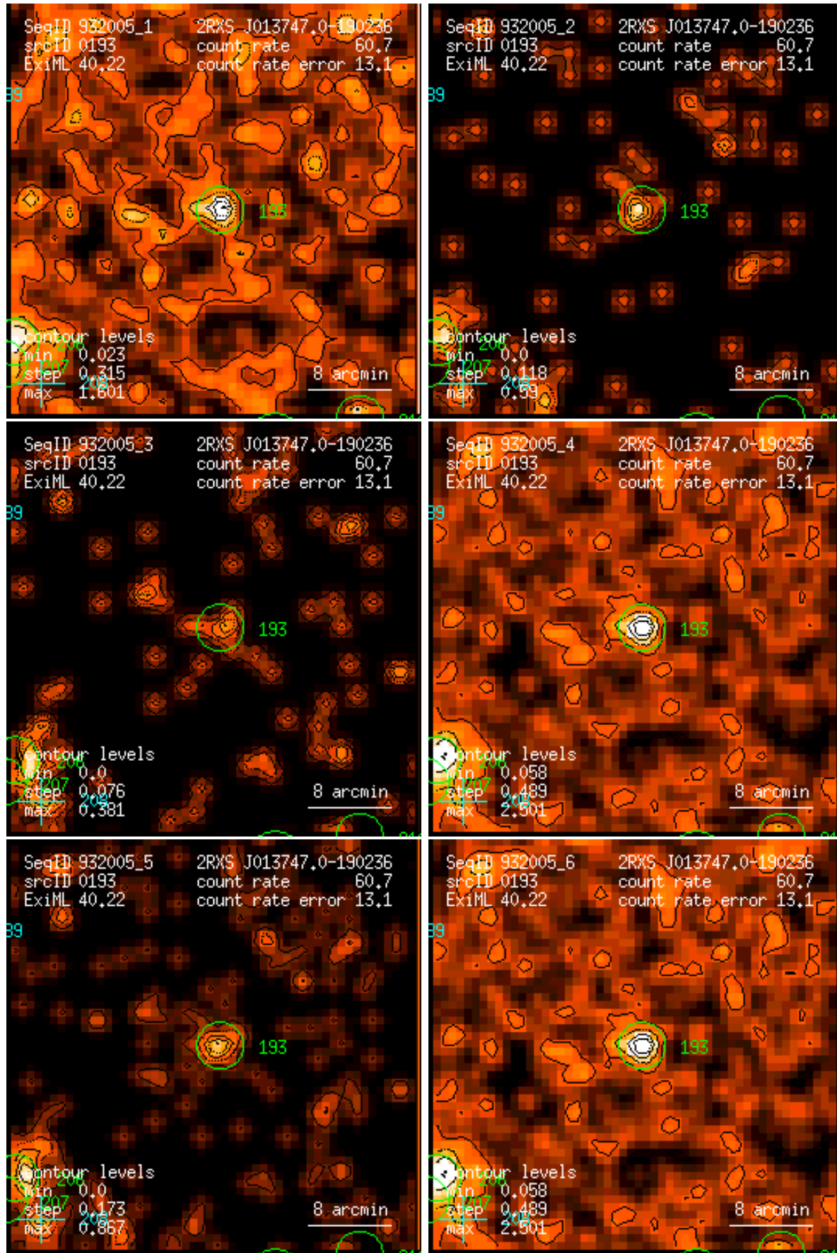
Figure 193: RASS 932005: detection 0193: band rate images, Gaussian filter: (1) PSPC channels 11 – 41, (2) 52 – 90, (3) 91 – 201, (4) 11 – 235, (5) 52 – 201, (6) 11 – 201. Broad band rates in counts/ks. Band rate contour levels in counts/ks/arcmin 2 .
