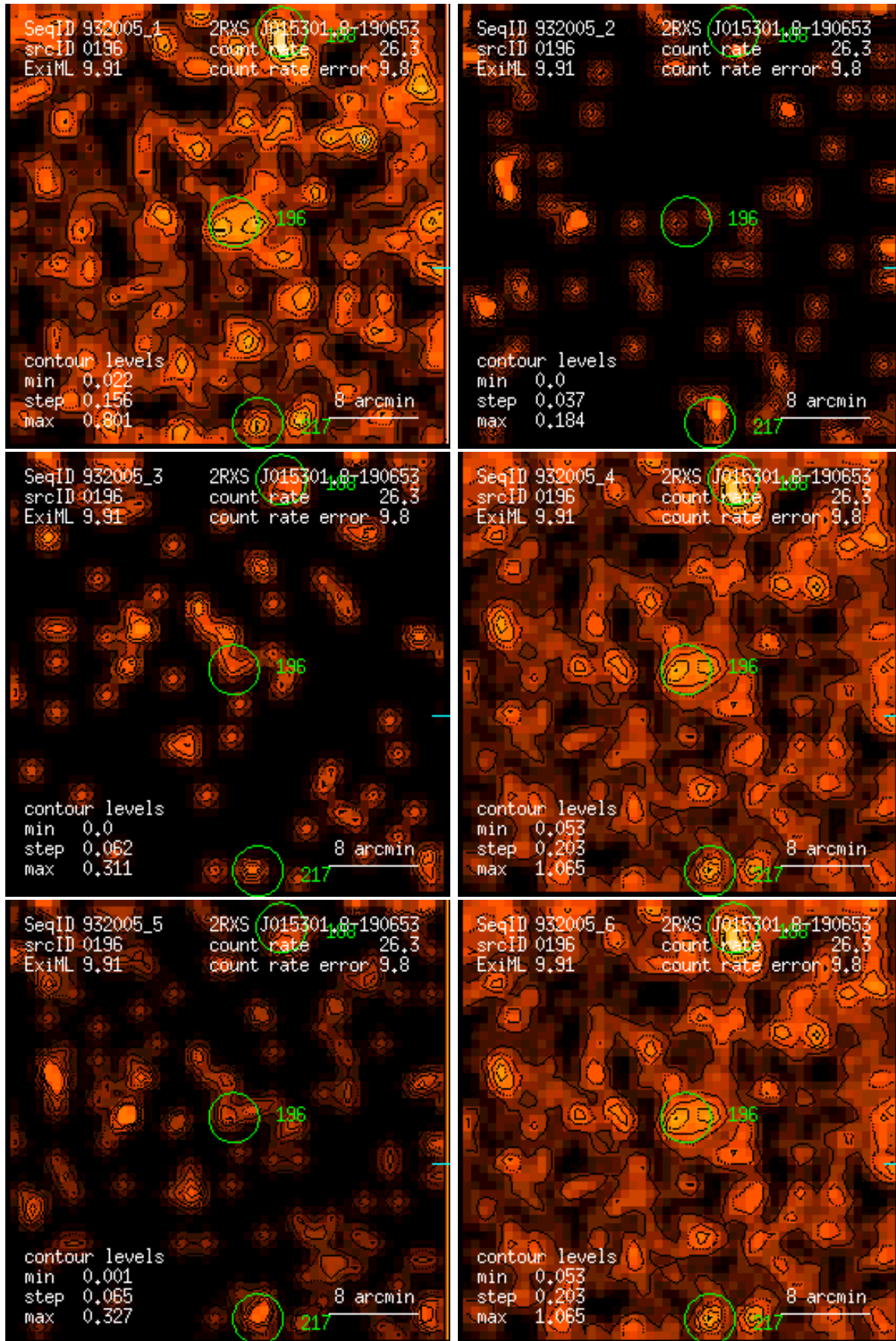
Figure 196: RASS 932005: detection 0196: band rate images, Gaussian filter: (1) PSPC channels 11 – 41, (2) 52 – 90, (3) 91 – 201, (4) 11 – 235, (5) 52 – 201, (6) 11 – 201. Broad band rates in counts/ks. Band rate contour levels in counts/ks/arcmin 2 .
