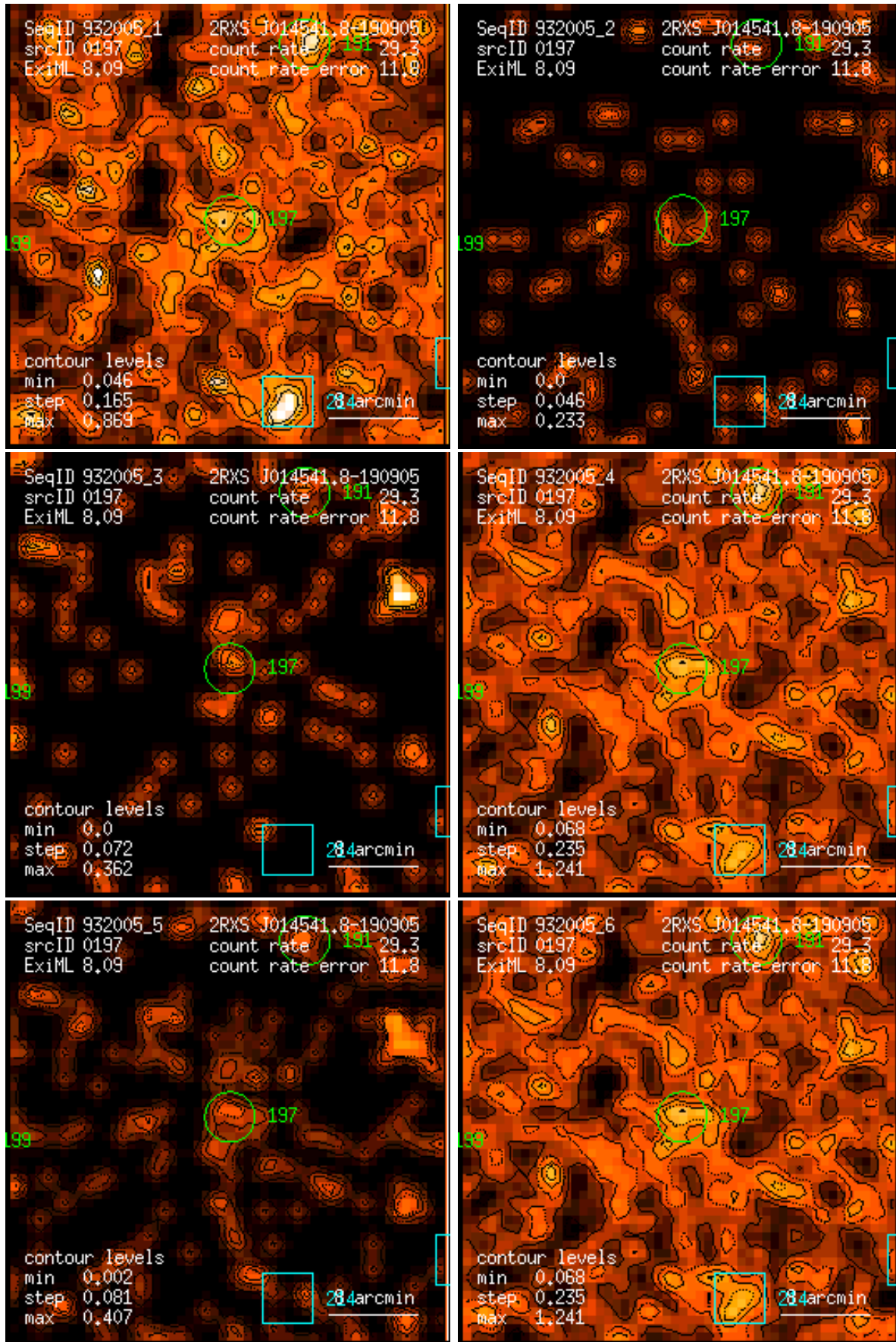
Figure 197: RASS 932005: detection 0197: band rate images, Gaussian filter: (1) PSPC channels 11 – 41, (2) 52 – 90, (3) 91 – 201, (4) 11 – 235, (5) 52 – 201, (6) 11 – 201. Broad band rates in counts/ks. Band rate contour levels in counts/ks/arcmin 2 .
