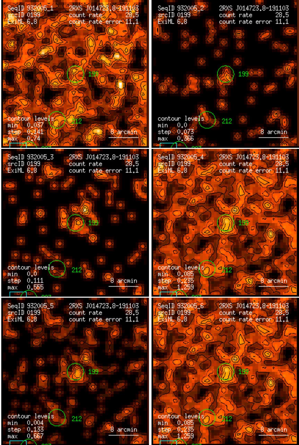
Figure 199: RASS 932005: detection 0199: band rate images, Gaussian filter: (1) PSPC channels 11 – 41, (2) 52 – 90, (3) 91 – 201, (4) 11 – 235, (5) 52 – 201, (6) 11 – 201. Broad band rates in counts/ks. Band rate contour levels in counts/ks/arcmin 2 .
