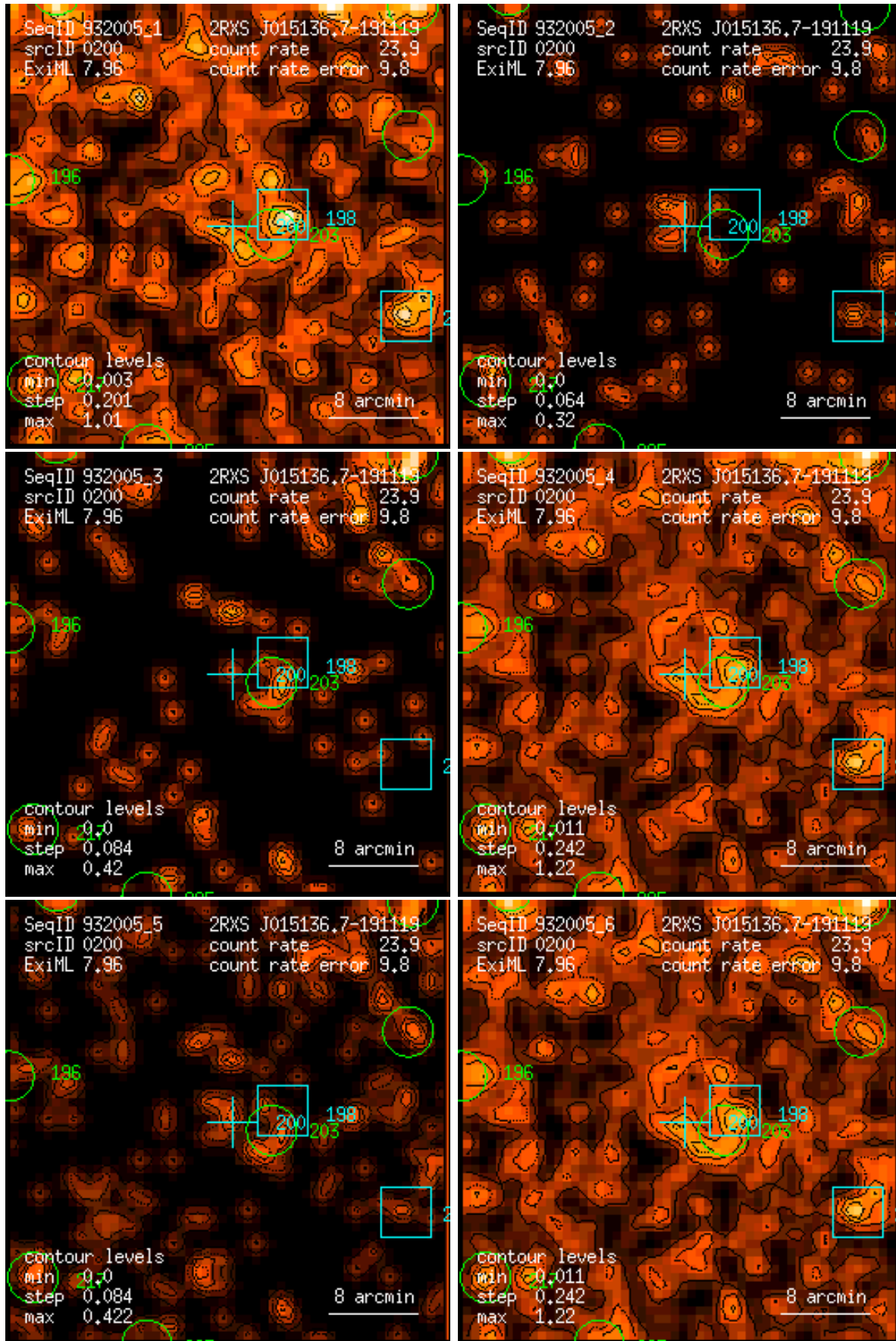
Figure 200: RASS 932005: detection 0200: band rate images, Gaussian filter: (1) PSPC channels 11 – 41, (2) 52 – 90, (3) 91 – 201, (4) 11 – 235, (5) 52 – 201, (6) 11 – 201. Broad band rates in counts/ks. Band rate contour levels in counts/ks/arcmin 2 .
