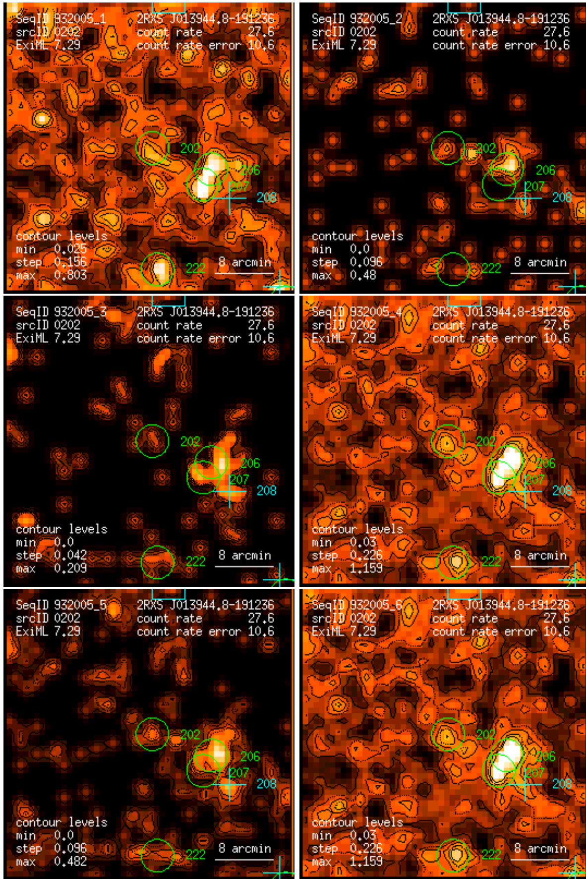
Figure 202: RASS 932005: detection 0202: band rate images, Gaussian filter: (1) PSPC channels 11 – 41, (2) 52 – 90, (3) 91 – 201, (4) 11 – 235, (5) 52 – 201, (6) 11 – 201. Broad band rates in counts/ks. Band rate contour levels in counts/ks/arcmin 2 .
