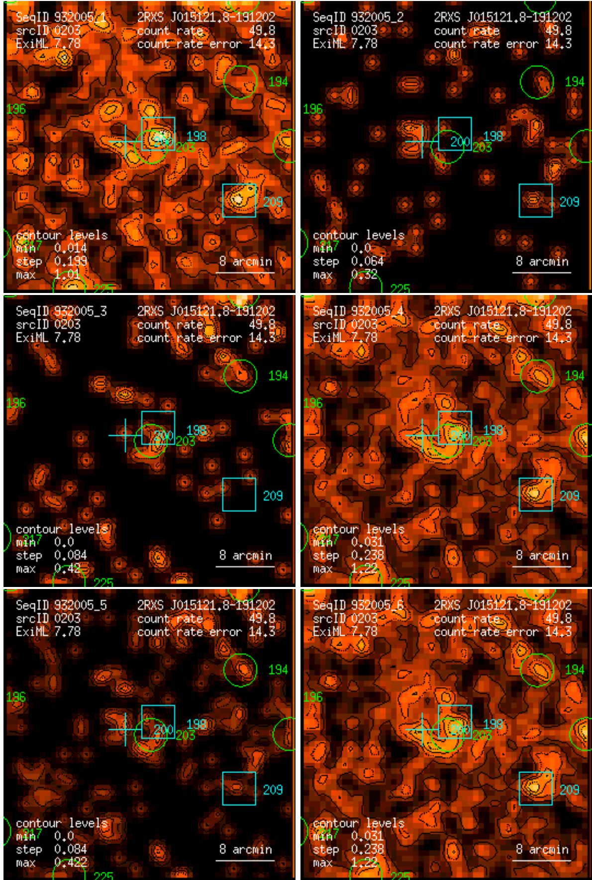
Figure 203: RASS 932005: detection 0203: band rate images, Gaussian filter: (1) PSPC channels 11 – 41, (2) 52 – 90, (3) 91 – 201, (4) 11 – 235, (5) 52 – 201, (6) 11 – 201. Broad band rates in counts/ks. Band rate contour levels in counts/ks/arcmin 2 .
