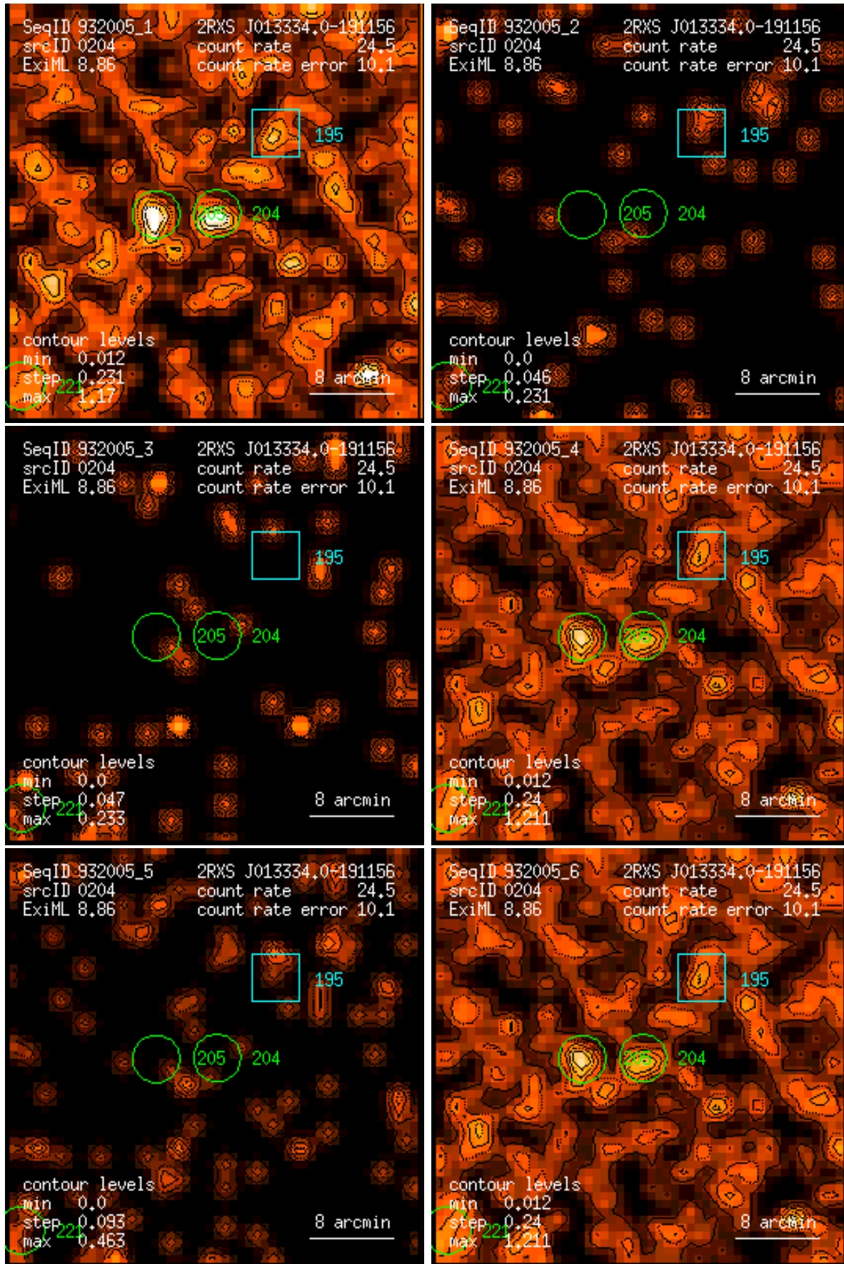
Figure 204: RASS 932005: detection 0204: band rate images, Gaussian filter: (1) PSPC channels 11 – 41, (2) 52 – 90, (3) 91 – 201, (4) 11 – 235, (5) 52 – 201, (6) 11 – 201. Broad band rates in counts/ks. Band rate contour levels in counts/ks/arcmin 2 .
