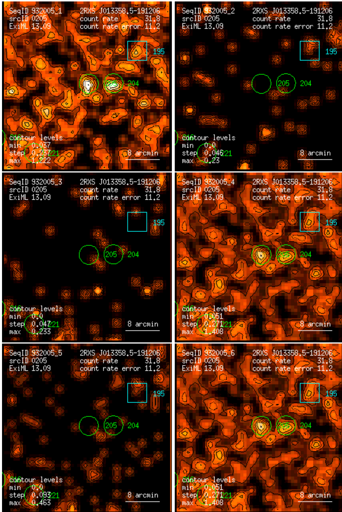
Figure 205: RASS 932005: detection 0205: band rate images, Gaussian filter: (1) PSPC channels 11 – 41, (2) 52 – 90, (3) 91 – 201, (4) 11 – 235, (5) 52 – 201, (6) 11 – 201. Broad band rates in counts/ks. Band rate contour levels in counts/ks/arcmin 2 .
