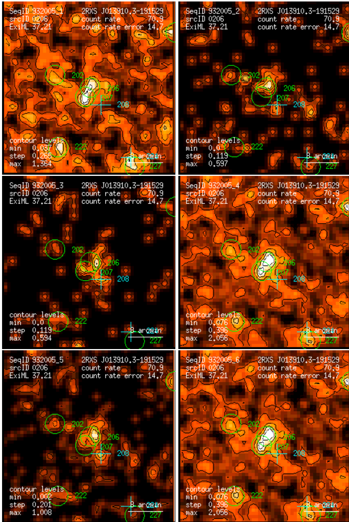
Figure 206: RASS 932005: detection 0206: band rate images, Gaussian filter: (1) PSPC channels 11 – 41, (2) 52 – 90, (3) 91 – 201, (4) 11 – 235, (5) 52 – 201, (6) 11 – 201. Broad band rates in counts/ks. Band rate contour levels in counts/ks/arcmin 2 .
