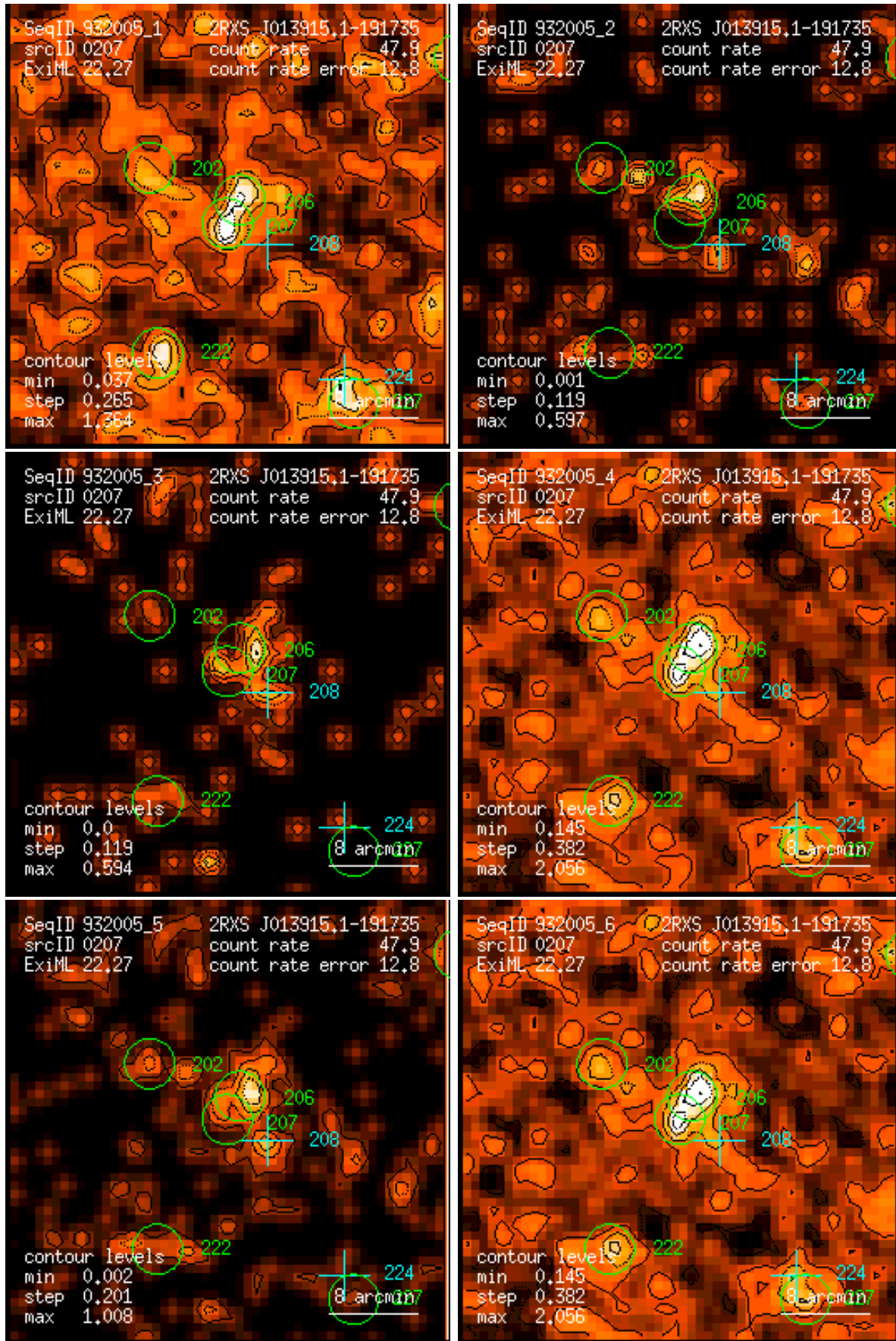
Figure 207: RASS 932005: detection 0207: band rate images, Gaussian filter: (1) PSPC channels 11 – 41, (2) 52 – 90, (3) 91 – 201, (4) 11 – 235, (5) 52 – 201, (6) 11 – 201. Broad band rates in counts/ks. Band rate contour levels in counts/ks/arcmin 2 .
