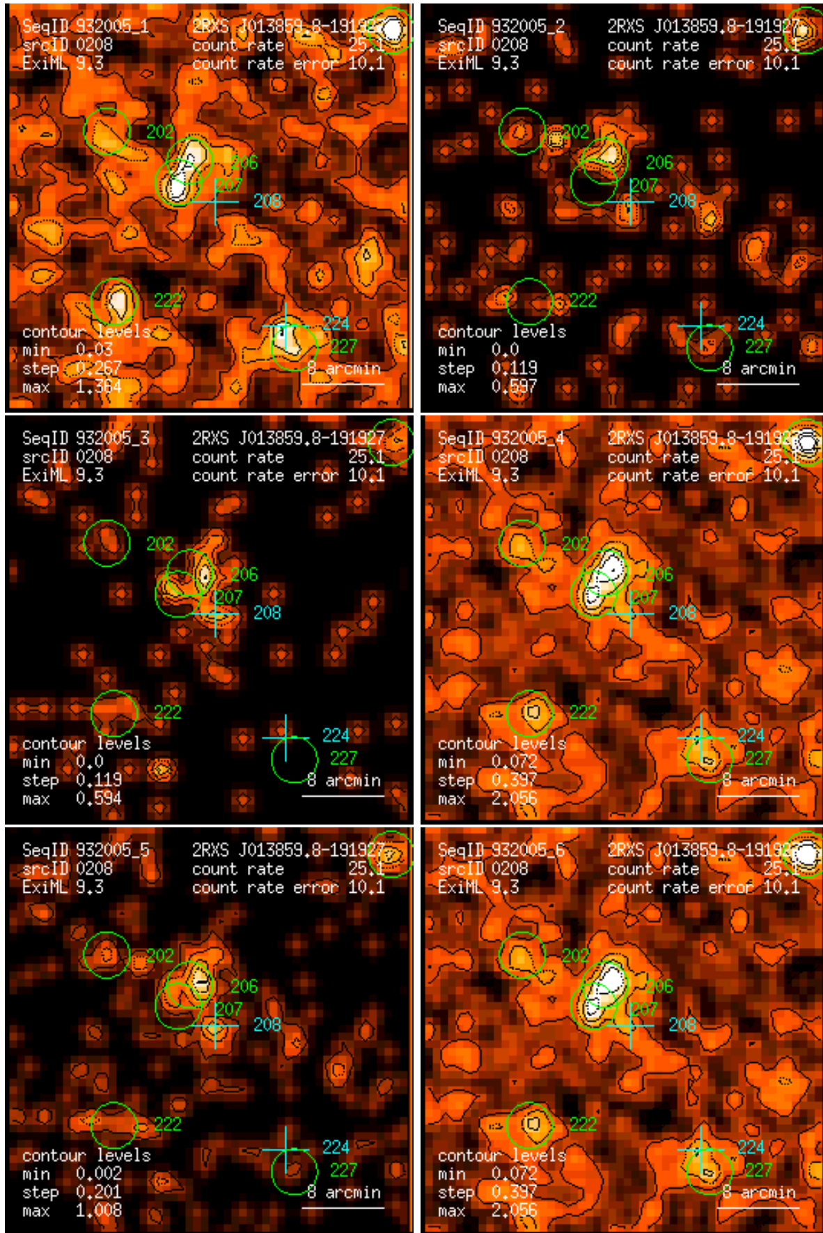
Figure 208: RASS 932005: detection 0208: band rate images, Gaussian filter: (1) PSPC channels 11 – 41, (2) 52 – 90, (3) 91 – 201, (4) 11 – 235, (5) 52 – 201, (6) 11 – 201. Broad band rates in counts/ks. Band rate contour levels in counts/ks/arcmin 2 .
