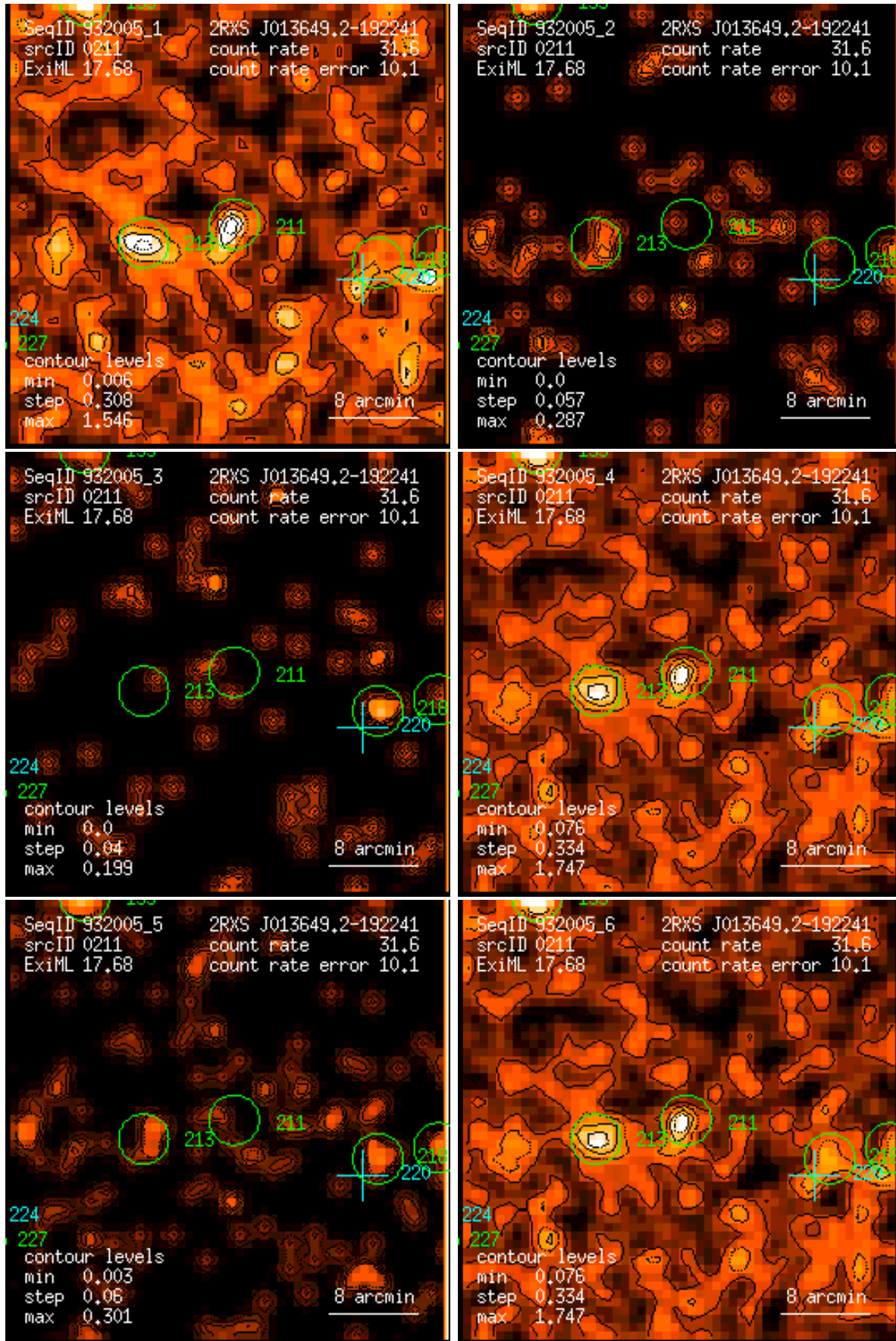
Figure 211: RASS 932005: detection 0211: band rate images, Gaussian filter: (1) PSPC channels 11 – 41, (2) 52 – 90, (3) 91 – 201, (4) 11 – 235, (5) 52 – 201, (6) 11 – 201. Broad band rates in counts/ks. Band rate contour levels in counts/ks/arcmin 2 .
