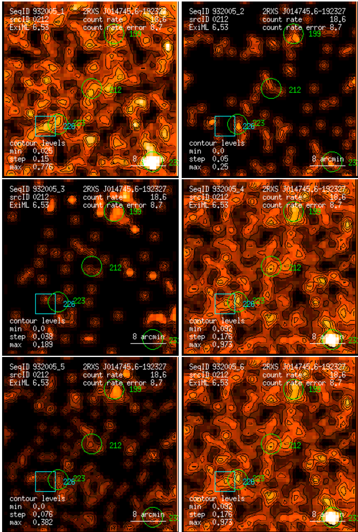
Figure 212: RASS 932005: detection 0212: band rate images, Gaussian filter: (1) PSPC channels 11 – 41, (2) 52 – 90, (3) 91 – 201, (4) 11 – 235, (5) 52 – 201, (6) 11 – 201. Broad band rates in counts/ks. Band rate contour levels in counts/ks/arcmin 2 .
