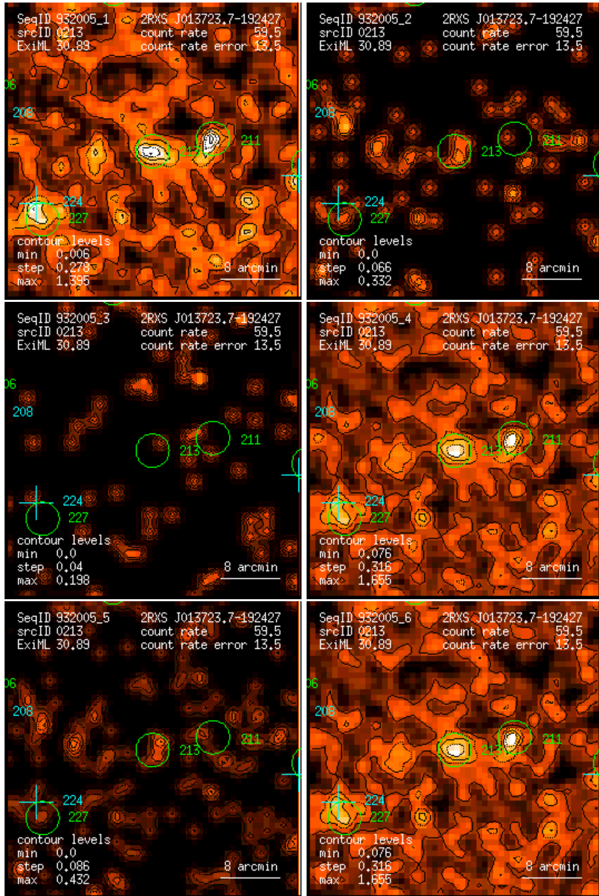
Figure 213: RASS 932005: detection 0213: band rate images, Gaussian filter: (1) PSPC channels 11 – 41, (2) 52 – 90, (3) 91 – 201, (4) 11 – 235, (5) 52 – 201, (6) 11 – 201. Broad band rates in counts/ks. Band rate contour levels in counts/ks/arcmin 2 .
