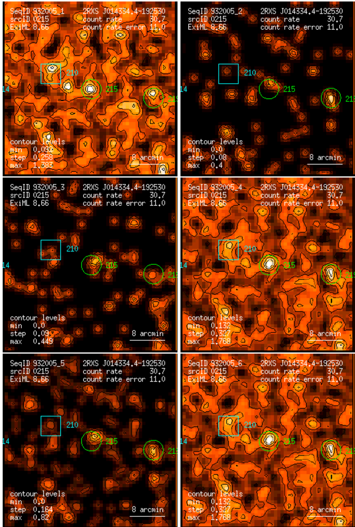
Figure 215: RASS 932005: detection 0215: band rate images, Gaussian filter: (1) PSPC channels 11 – 41, (2) 52 – 90, (3) 91 – 201, (4) 11 – 235, (5) 52 – 201, (6) 11 – 201. Broad band rates in counts/ks. Band rate contour levels in counts/ks/arcmin 2 .
