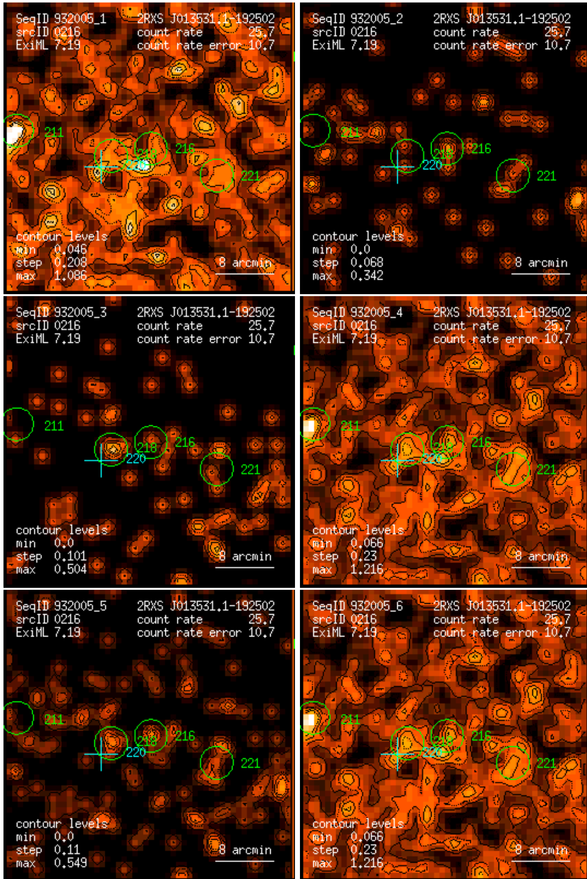
Figure 216: RASS 932005: detection 0216: band rate images, Gaussian filter: (1) PSPC channels 11 – 41, (2) 52 – 90, (3) 91 – 201, (4) 11 – 235, (5) 52 – 201, (6) 11 – 201. Broad band rates in counts/ks. Band rate contour levels in counts/ks/arcmin 2 .
