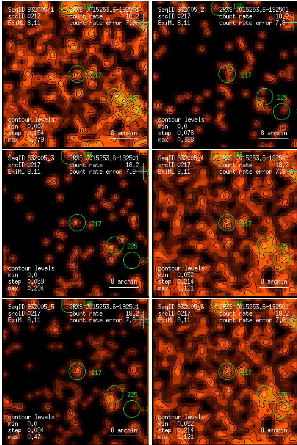
Figure 217: RASS 932005: detection 0217: band rate images, Gaussian filter: (1) PSPC channels 11 – 41, (2) 52 – 90, (3) 91 – 201, (4) 11 – 235, (5) 52 – 201, (6) 11 – 201. Broad band rates in counts/ks. Band rate contour levels in counts/ks/arcmin 2 .
