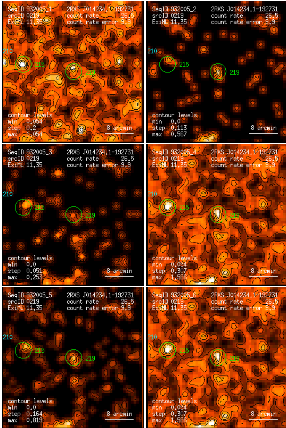
Figure 219: RASS 932005: detection 0219: band rate images, Gaussian filter: (1) PSPC channels 11 – 41, (2) 52 – 90, (3) 91 – 201, (4) 11 – 235, (5) 52 – 201, (6) 11 – 201. Broad band rates in counts/ks. Band rate contour levels in counts/ks/arcmin 2 .
