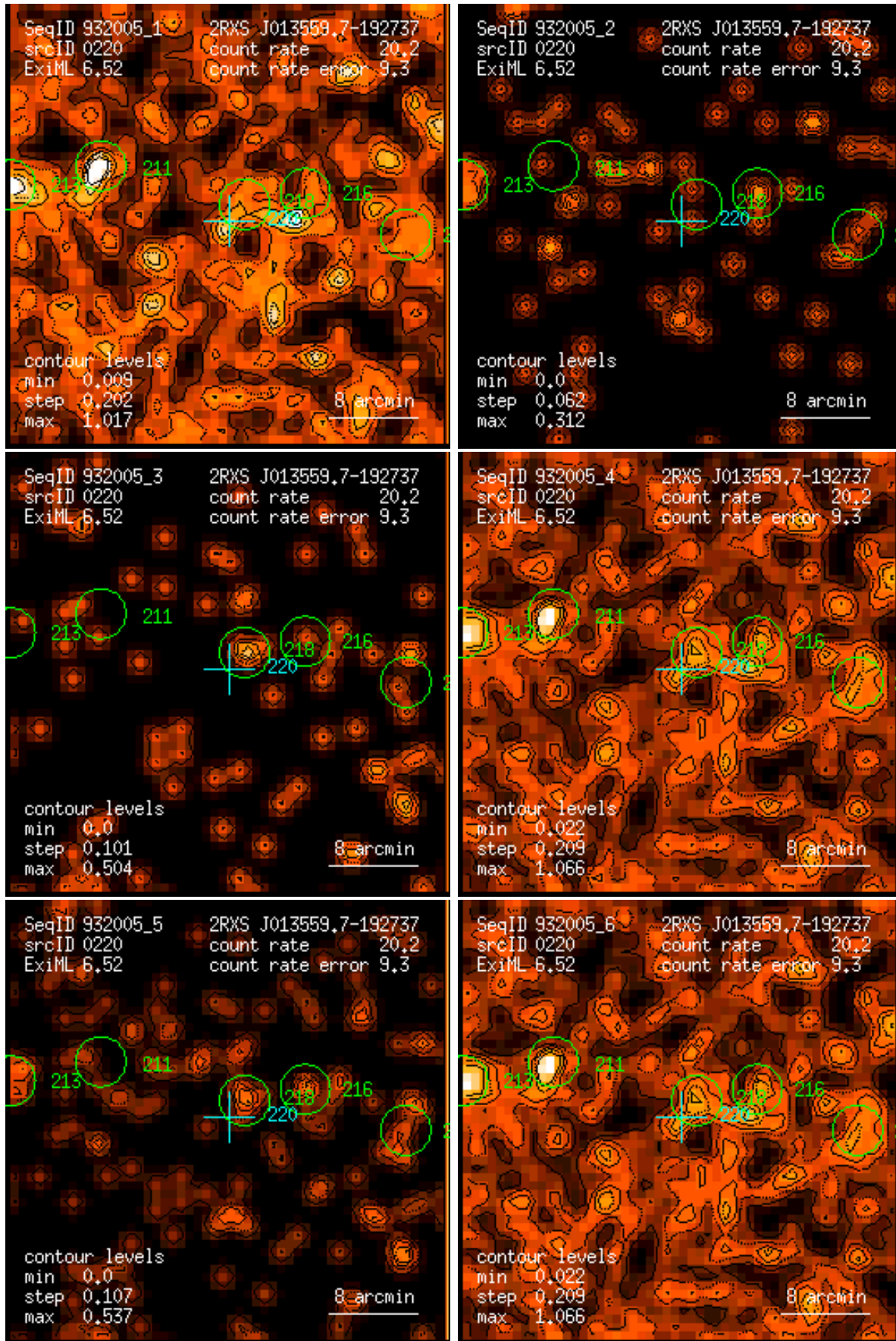
Figure 220: RASS 932005: detection 0220: band rate images, Gaussian filter: (1) PSPC channels 11 – 41, (2) 52 – 90, (3) 91 – 201, (4) 11 – 235, (5) 52 – 201, (6) 11 – 201. Broad band rates in counts/ks. Band rate contour levels in counts/ks/arcmin 2 .
