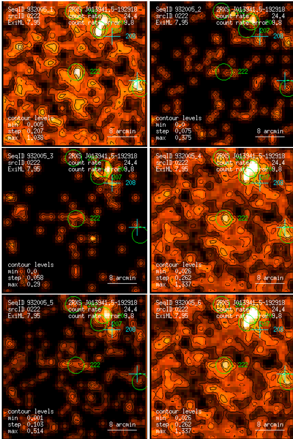
Figure 222: RASS 932005: detection 0222: band rate images, Gaussian filter: (1) PSPC channels 11 – 41, (2) 52 – 90, (3) 91 – 201, (4) 11 – 235, (5) 52 – 201, (6) 11 – 201. Broad band rates in counts/ks. Band rate contour levels in counts/ks/arcmin 2 .
