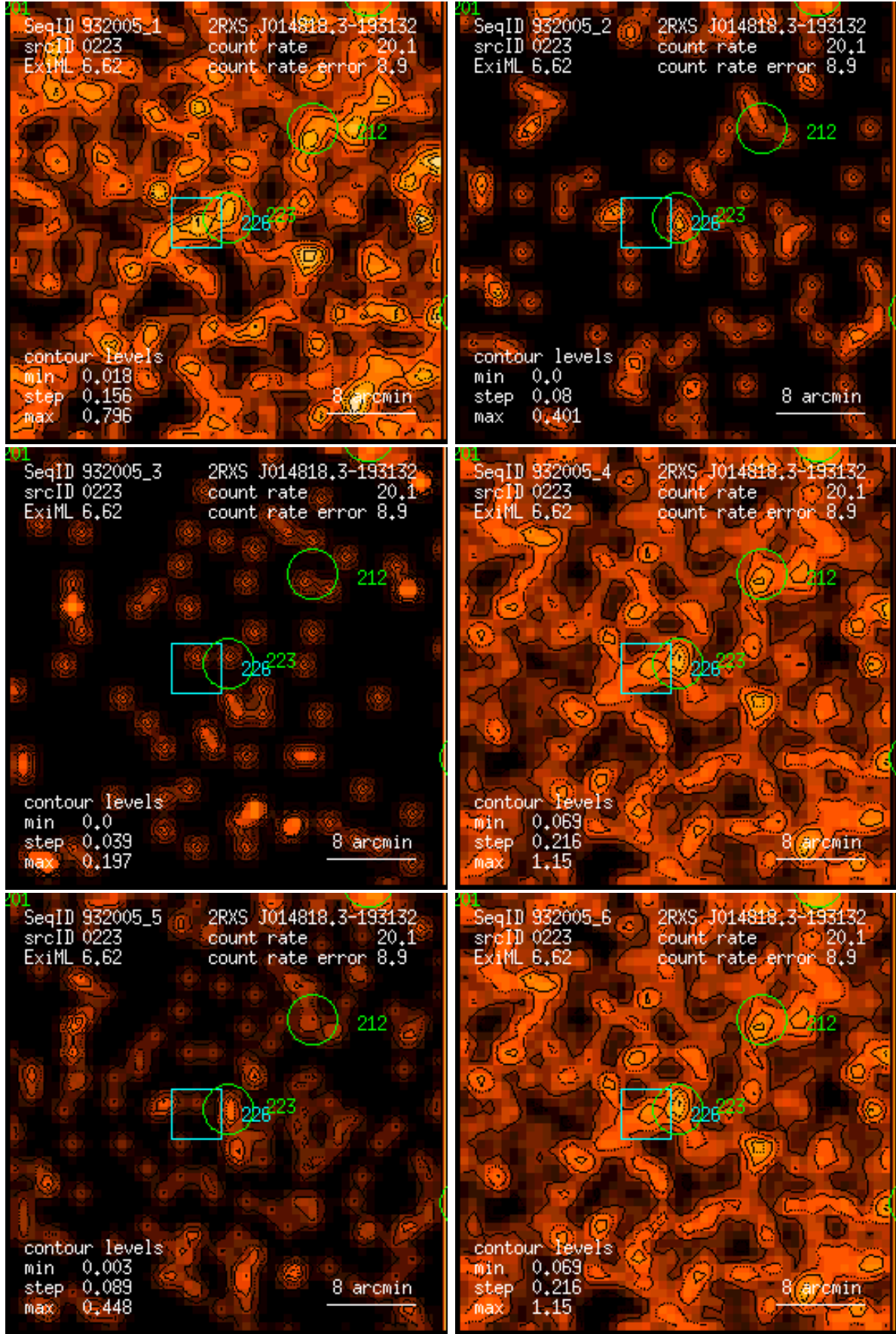
Figure 223: RASS 932005: detection 0223: band rate images, Gaussian filter: (1) PSPC channels 11 – 41, (2) 52 – 90, (3) 91 – 201, (4) 11 – 235, (5) 52 – 201, (6) 11 – 201. Broad band rates in counts/ks. Band rate contour levels in counts/ks/arcmin 2 .
