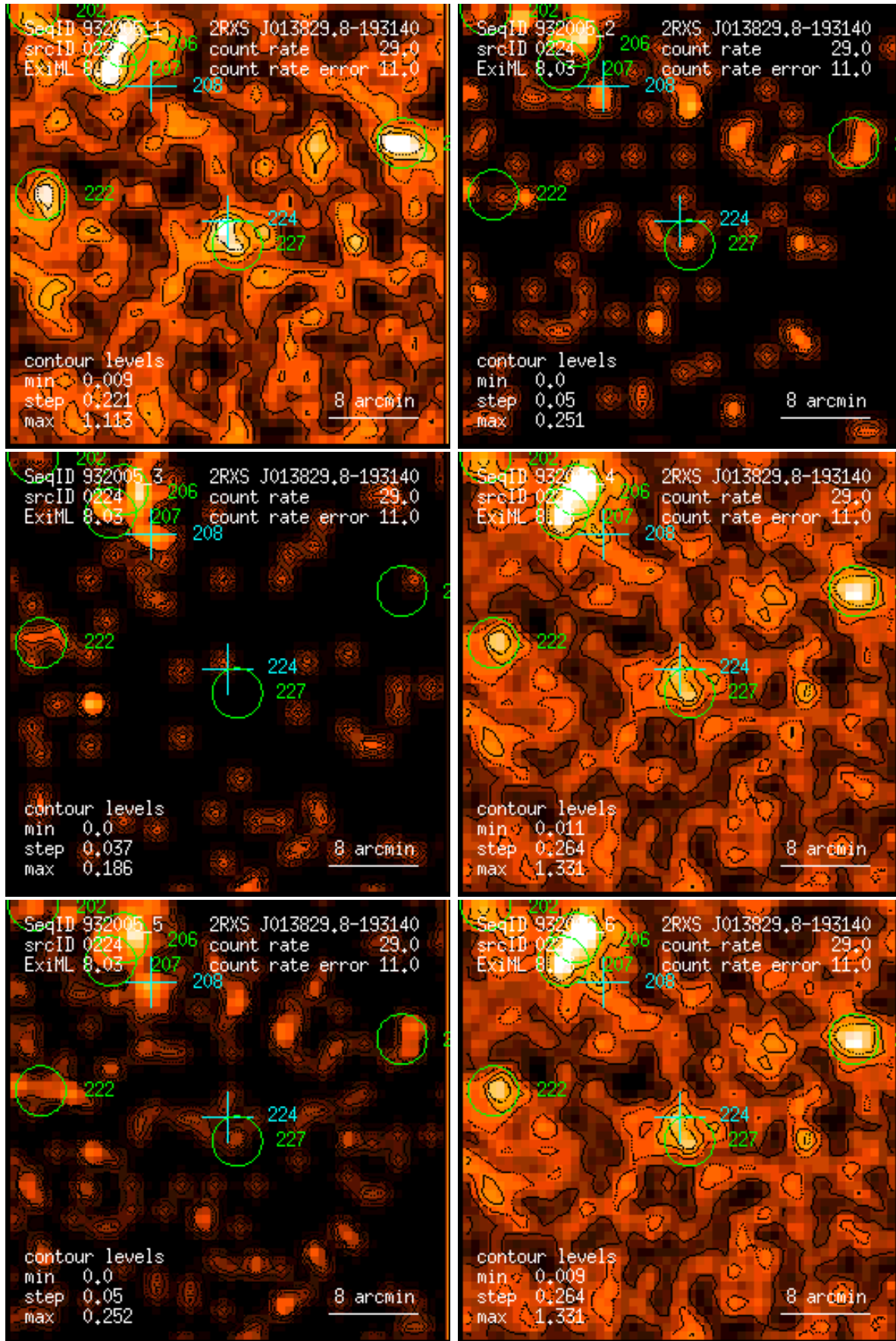
Figure 224: RASS 932005: detection 0224: band rate images, Gaussian filter: (1) PSPC channels 11 – 41, (2) 52 – 90, (3) 91 – 201, (4) 11 – 235, (5) 52 – 201, (6) 11 – 201. Broad band rates in counts/ks. Band rate contour levels in counts/ks/arcmin 2 .
