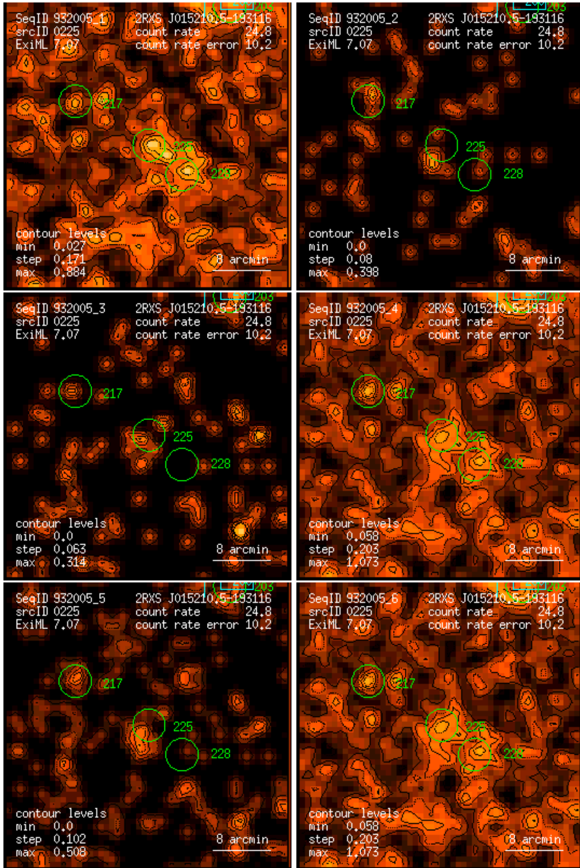
Figure 225: RASS 932005: detection 0225: band rate images, Gaussian filter: (1) PSPC channels 11 – 41, (2) 52 – 90, (3) 91 – 201, (4) 11 – 235, (5) 52 – 201, (6) 11 – 201. Broad band rates in counts/ks. Band rate contour levels in counts/ks/arcmin 2 .
