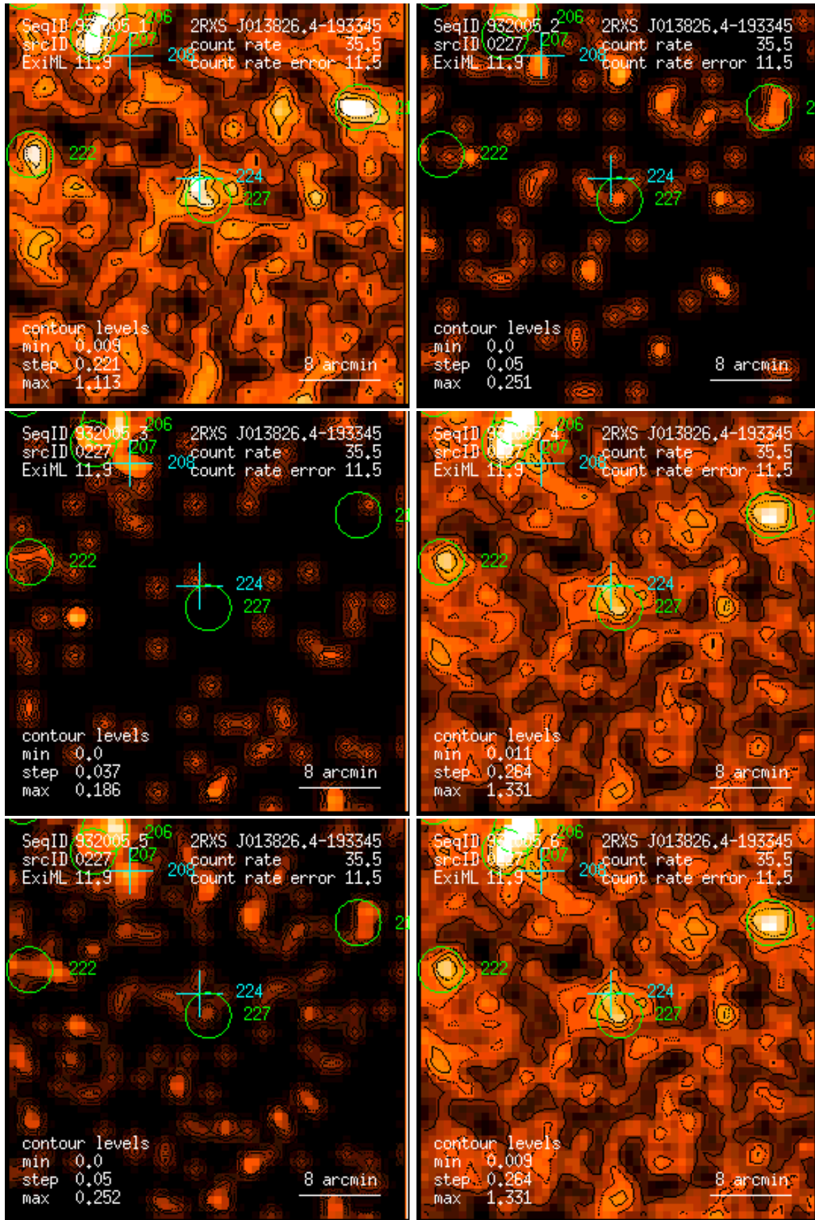
Figure 227: RASS 932005: detection 0227: band rate images, Gaussian filter: (1) PSPC channels 11 – 41, (2) 52 – 90, (3) 91 – 201, (4) 11 – 235, (5) 52 – 201, (6) 11 – 201. Broad band rates in counts/ks. Band rate contour levels in counts/ks/arcmin 2 .
