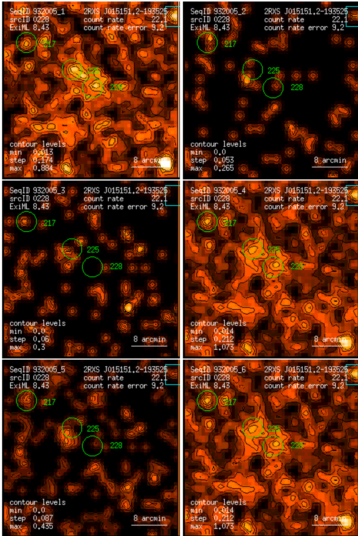
Figure 228: RASS 932005: detection 0228: band rate images, Gaussian filter: (1) PSPC channels 11 – 41, (2) 52 – 90, (3) 91 – 201, (4) 11 – 235, (5) 52 – 201, (6) 11 – 201. Broad band rates in counts/ks. Band rate contour levels in counts/ks/arcmin 2 .
