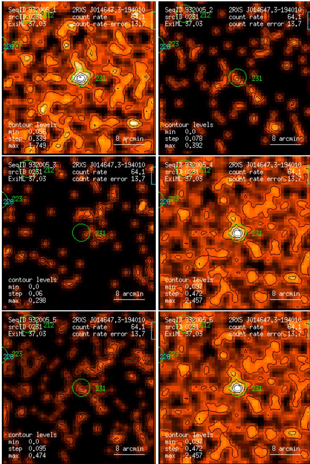
Figure 231: RASS 932005: detection 0231: band rate images, Gaussian filter: (1) PSPC channels 11 – 41, (2) 52 – 90, (3) 91 – 201, (4) 11 – 235, (5) 52 – 201, (6) 11 – 201. Broad band rates in counts/ks. Band rate contour levels in counts/ks/arcmin 2 .
