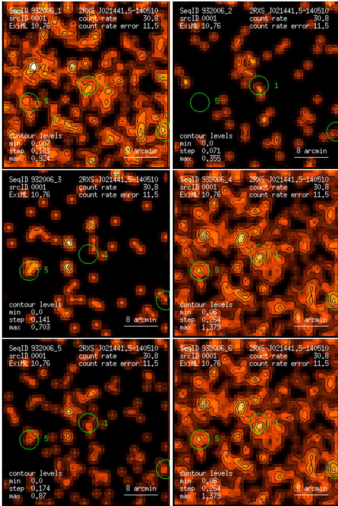
Figure 1: RASS 932006: detection 0001: band rate images, Gaussian filter: (1) PSPC channels 11 – 41, (2) 52 – 90, (3) 91 – 201, (4) 11 – 235, (5) 52 – 201, (6) 11 – 201. Broad band rates in counts/ks. Band rate contour levels in counts/ks/arcmin 2 .
