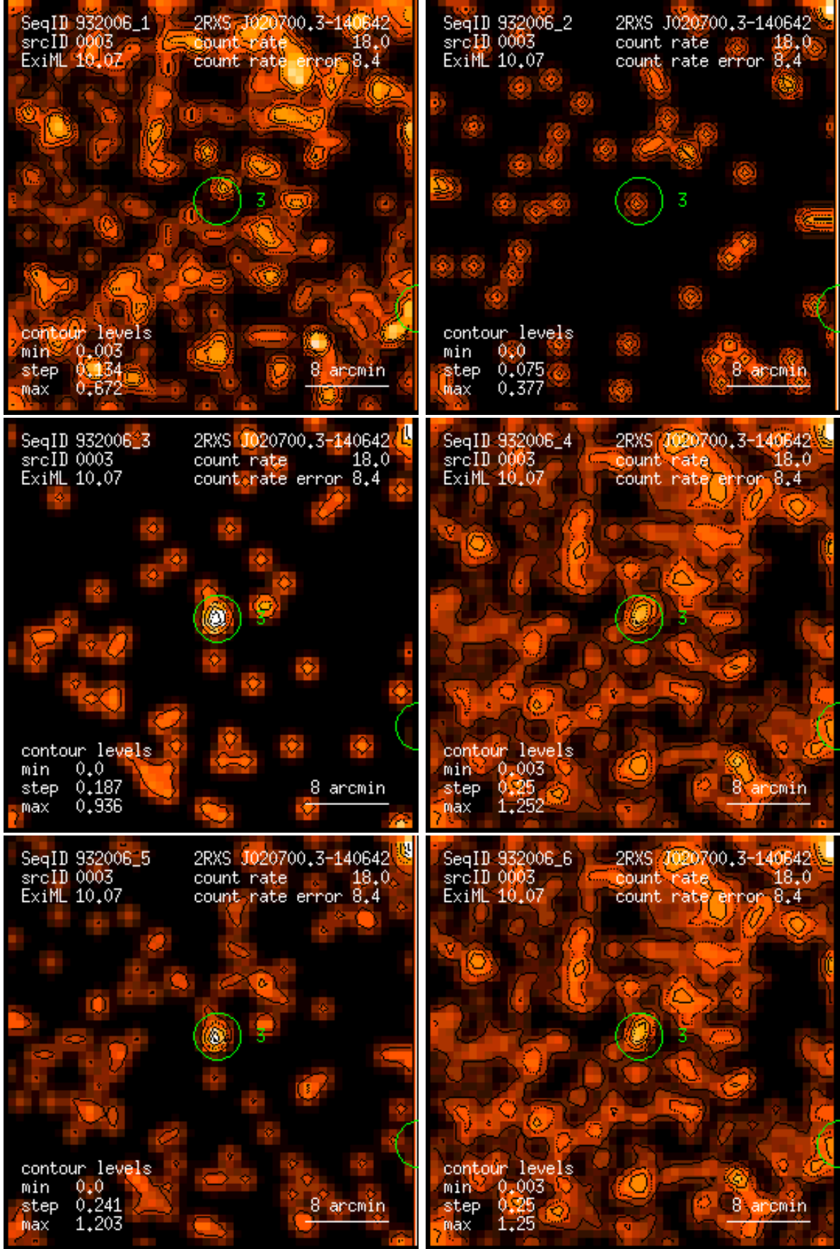
Figure 3: RASS 932006: detection 0003: band rate images, Gaussian filter: (1) PSPC channels 11 – 41, (2) 52 – 90, (3) 91 – 201, (4) 11 – 235, (5) 52 – 201, (6) 11 – 201. Broad band rates in counts/ks. Band rate contour levels in counts/ks/arcmin 2 .
