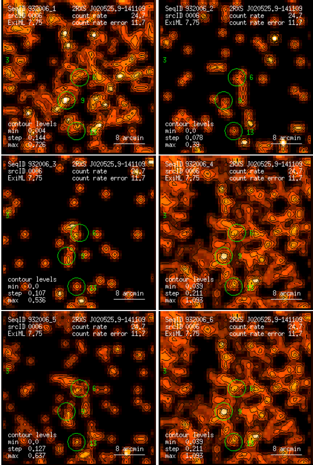
Figure 6: RASS 932006: detection 0006: band rate images, Gaussian filter: (1) PSPC channels 11 – 41, (2) 52 – 90, (3) 91 – 201, (4) 11 – 235, (5) 52 – 201, (6) 11 – 201. Broad band rates in counts/ks. Band rate contour levels in counts/ks/arcmin 2 .
