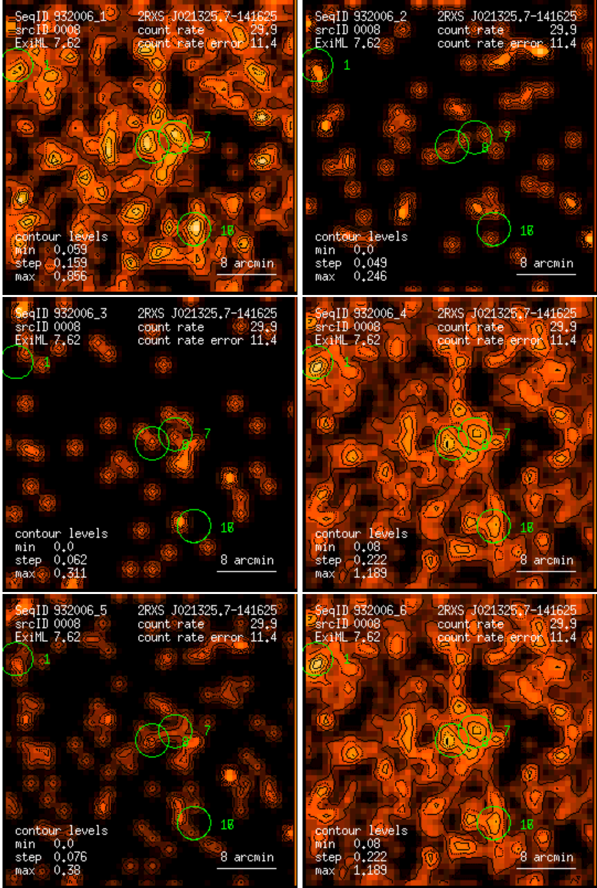
Figure 8: RASS 932006: detection 0008: band rate images, Gaussian filter: (1) PSPC channels 11 – 41, (2) 52 – 90, (3) 91 – 201, (4) 11 – 235, (5) 52 – 201, (6) 11 – 201. Broad band rates in counts/ks. Band rate contour levels in counts/ks/arcmin 2 .
