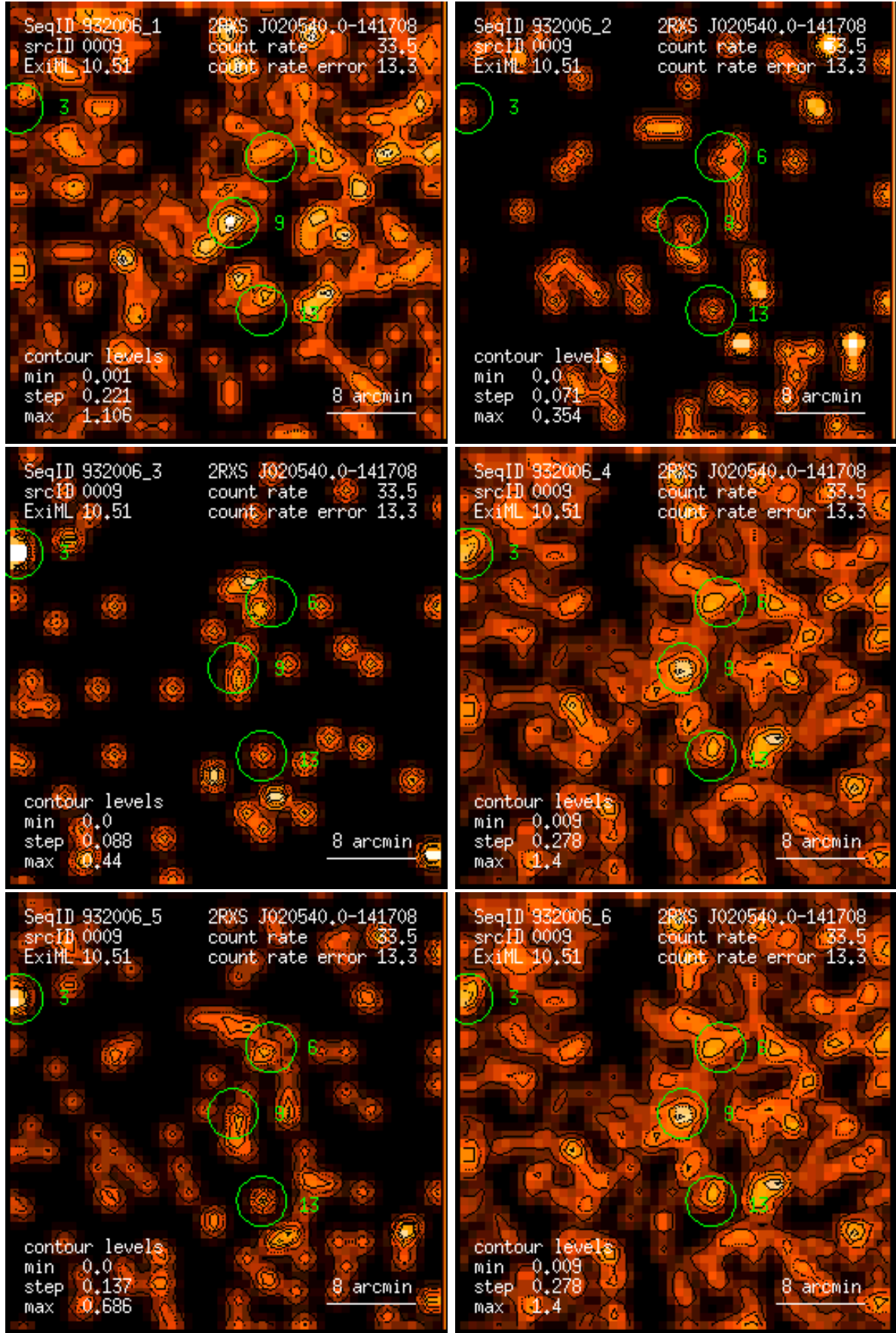
Figure 9: RASS 932006: detection 0009: band rate images, Gaussian filter: (1) PSPC channels 11 – 41, (2) 52 – 90, (3) 91 – 201, (4) 11 – 235, (5) 52 – 201, (6) 11 – 201. Broad band rates in counts/ks. Band rate contour levels in counts/ks/arcmin 2 .
